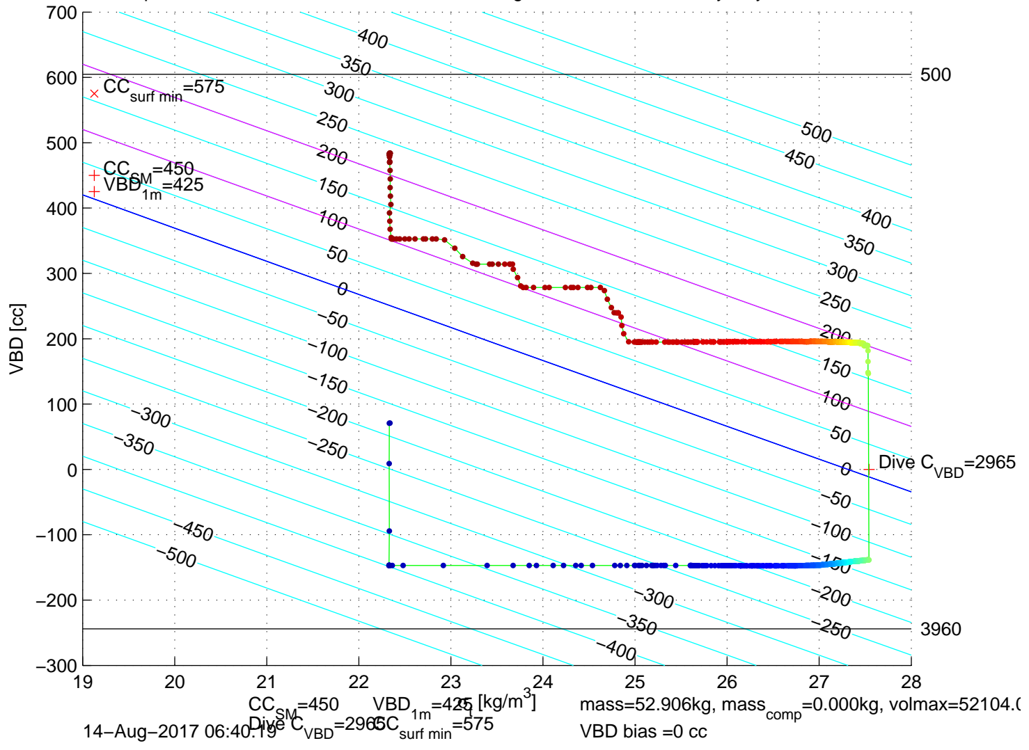
p6100192: SG610 Mission 7 Jul 2017 14-Aug-2017 06:10:45Z – buoyancy contoured
