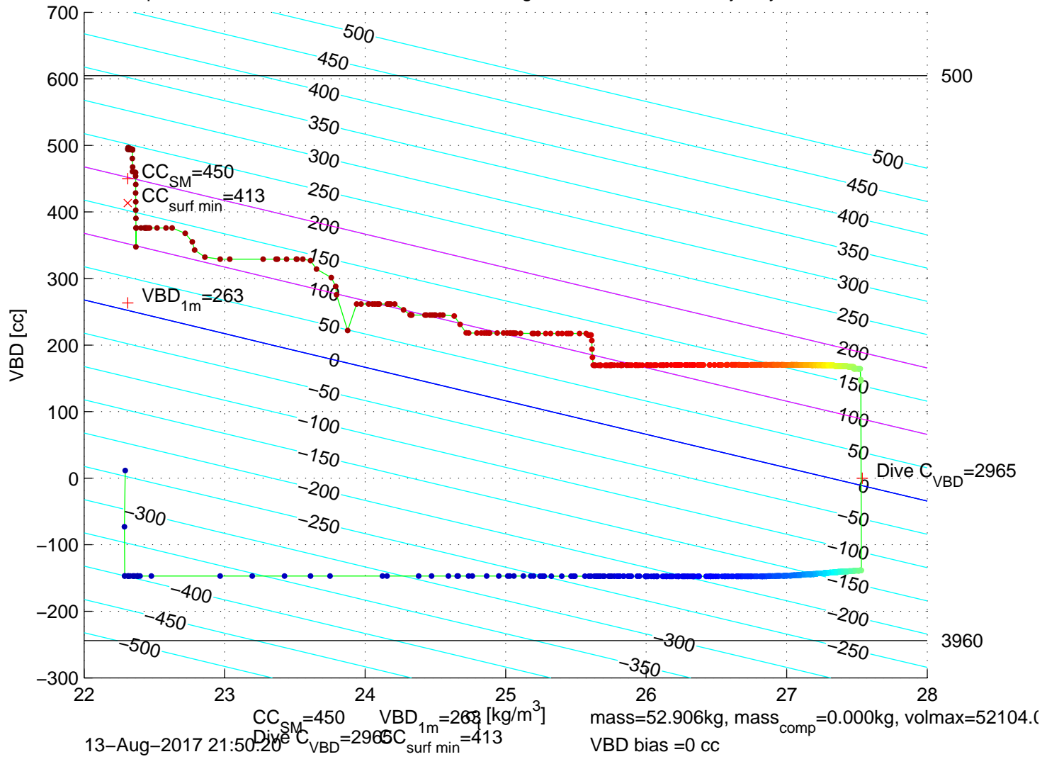
p6100190: SG610 Mission 7 Jul 2017 13-Aug-2017 21:17:50Z – buoyancy contoured
