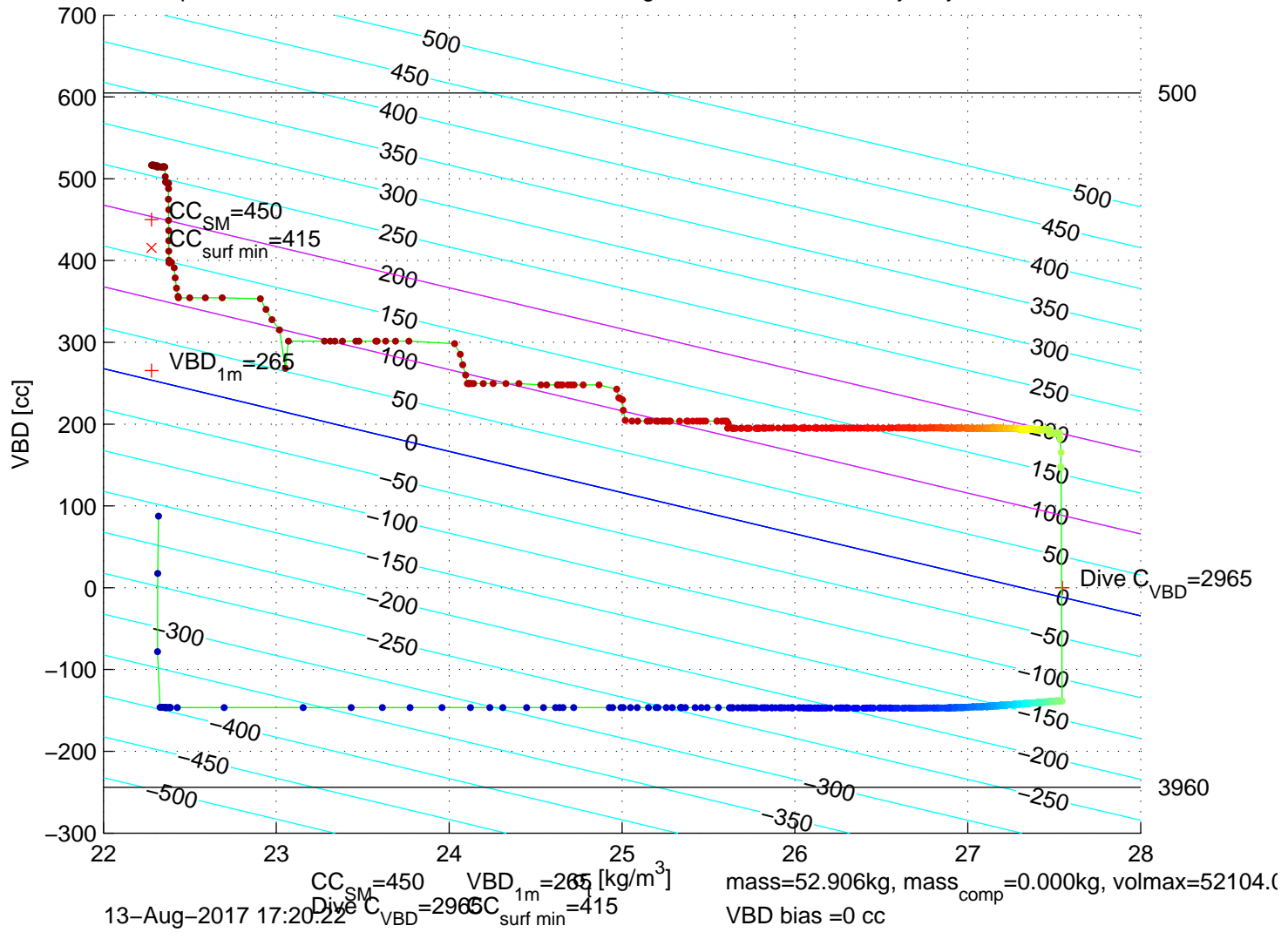
p6100189: SG610 Mission 7 Jul 2017 13-Aug-2017 17:02:05Z – buoyancy contoured
