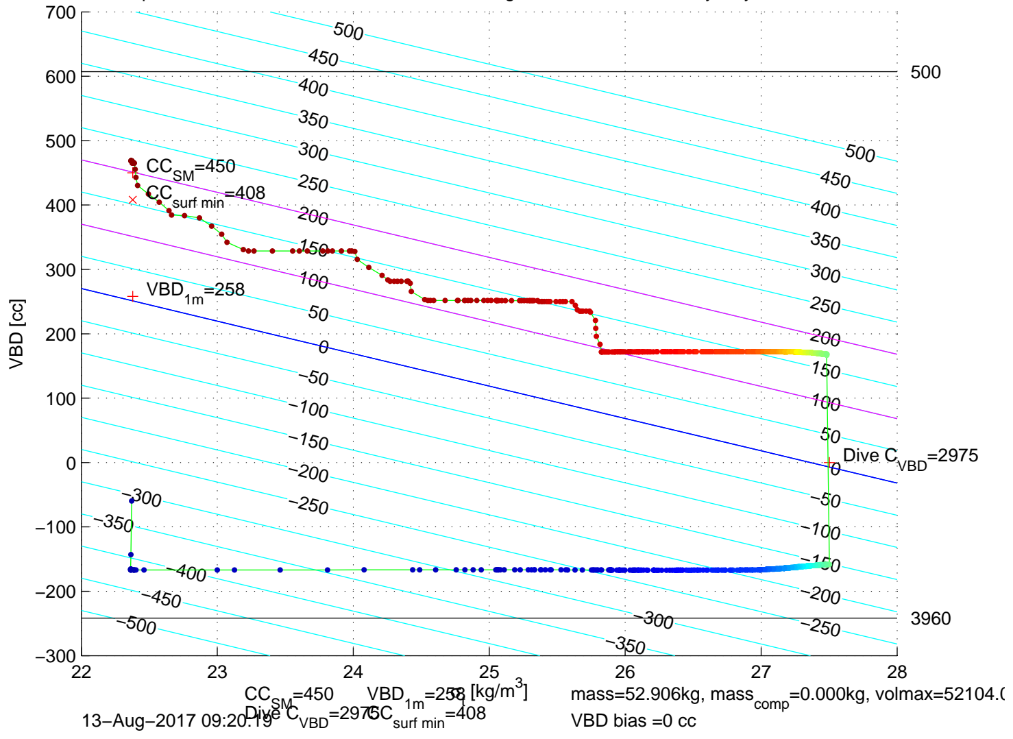
p6100187: SG610 Mission 7 Jul 2017 13-Aug-2017 08:45:08Z – buoyancy contoured
