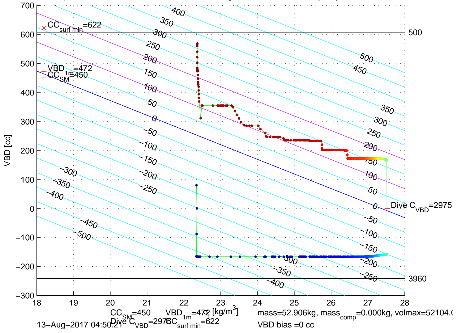
p6100186: SG610 Mission 7 Jul 2017 13-Aug-2017 04:17:35Z – buoyancy contoured
