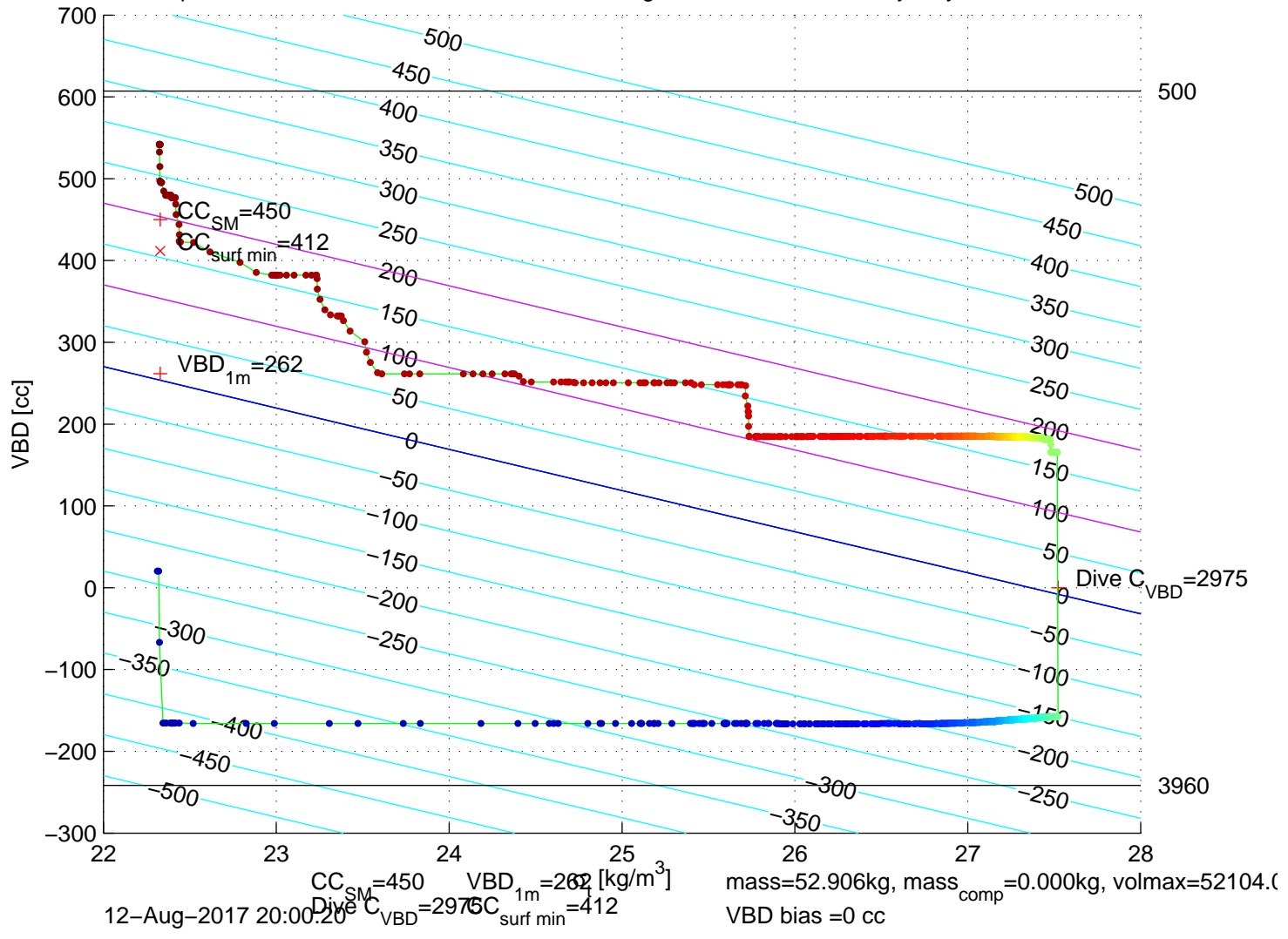
p6100184: SG610 Mission 7 Jul 2017 12-Aug-2017 19:24:02Z – buoyancy contoured
