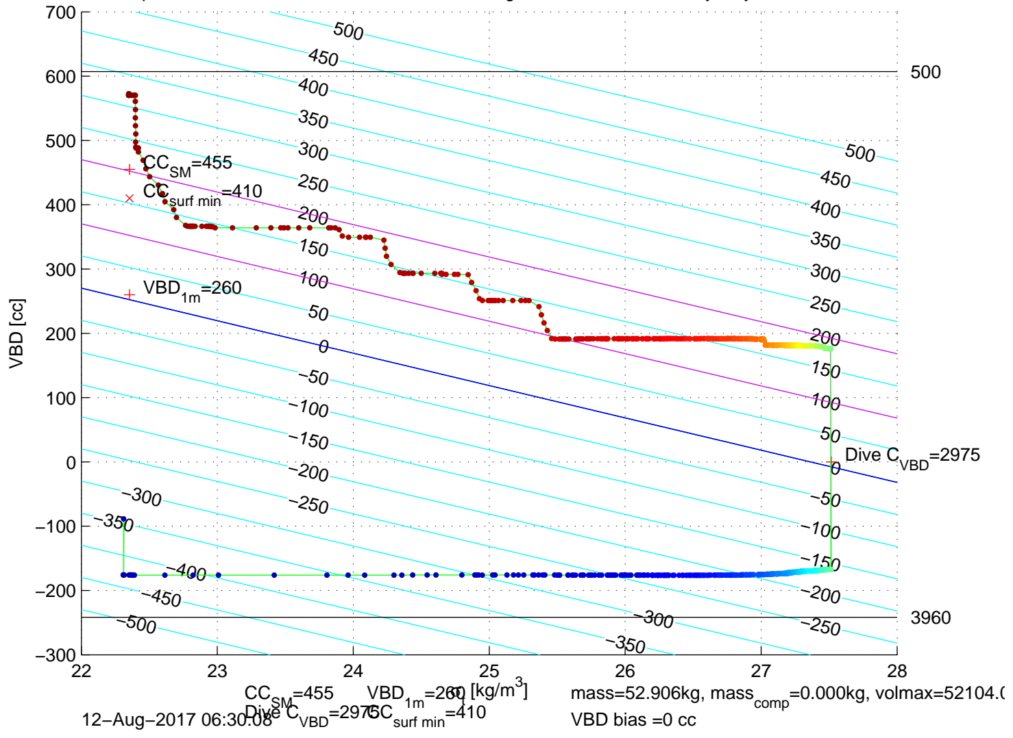
p6100181: SG610 Mission 7 Jul 2017 12-Aug-2017 06:07:13Z – buoyancy contoured
