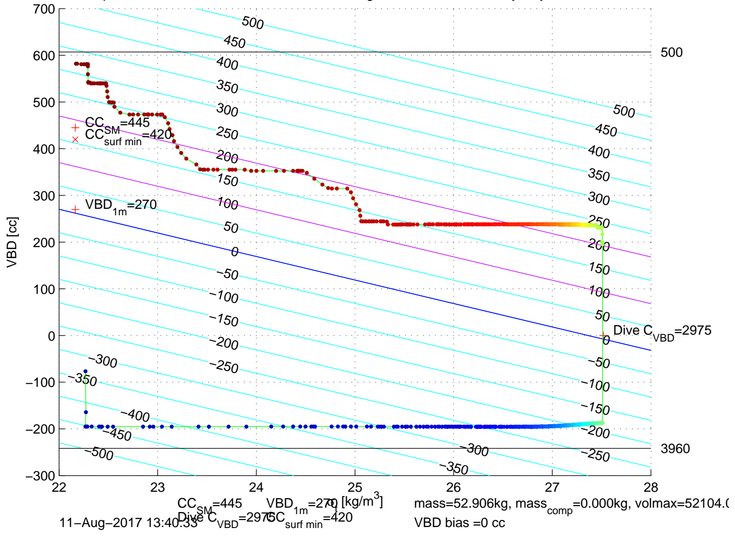
p6100177: SG610 Mission 7 Jul 2017 11–Aug–2017 13:25:05Z – buoyancy contoured
