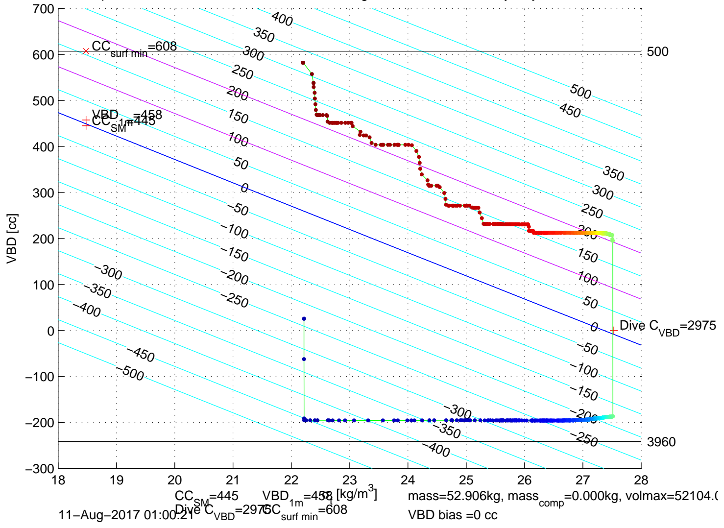
p6100174: SG610 Mission 7 Jul 2017 11-Aug-2017 00:29:20Z – buoyancy contoured
