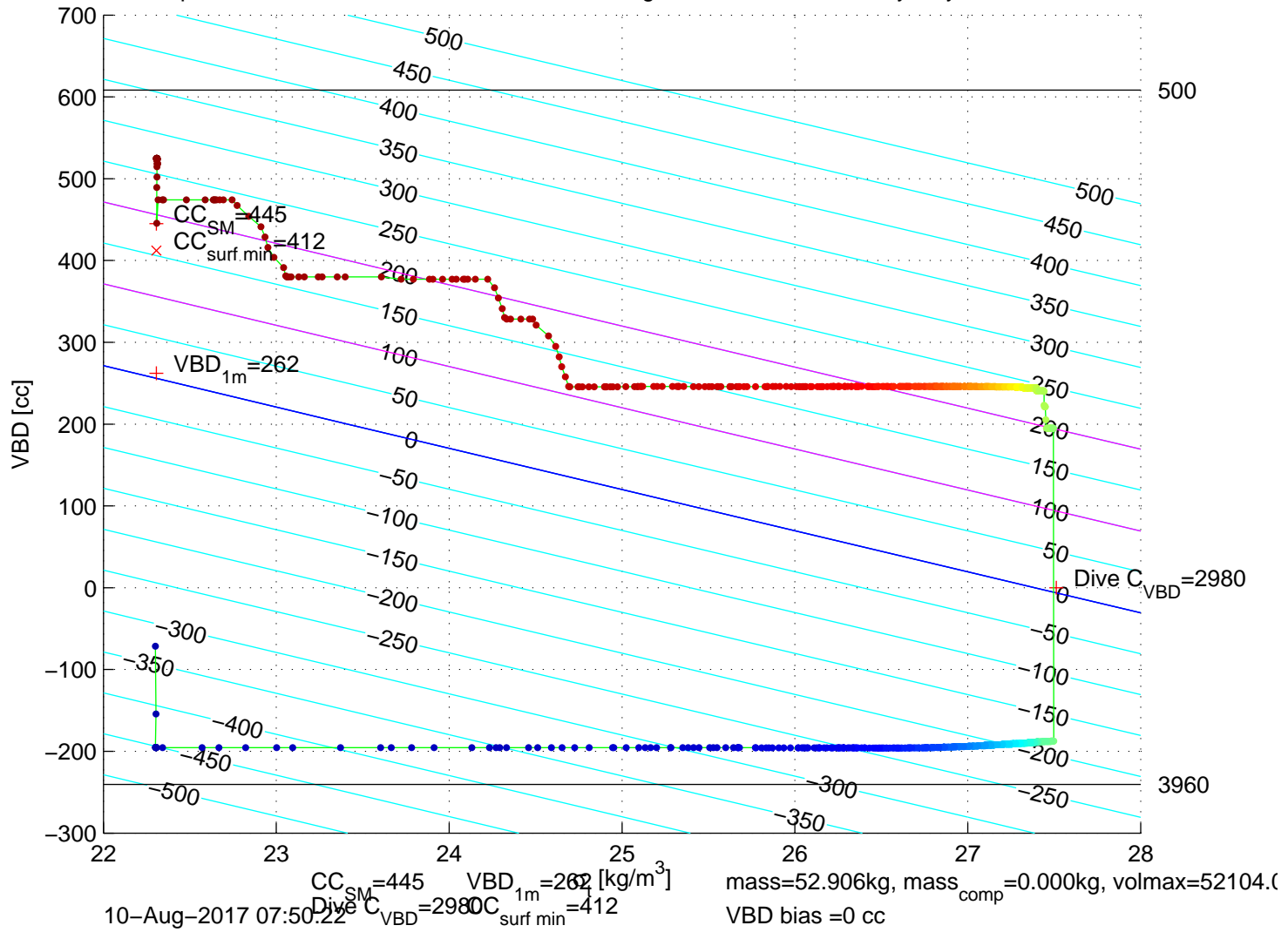
p6100170: SG610 Mission 7 Jul 2017 10–Aug–2017 07:31:12Z – buoyancy contoured
