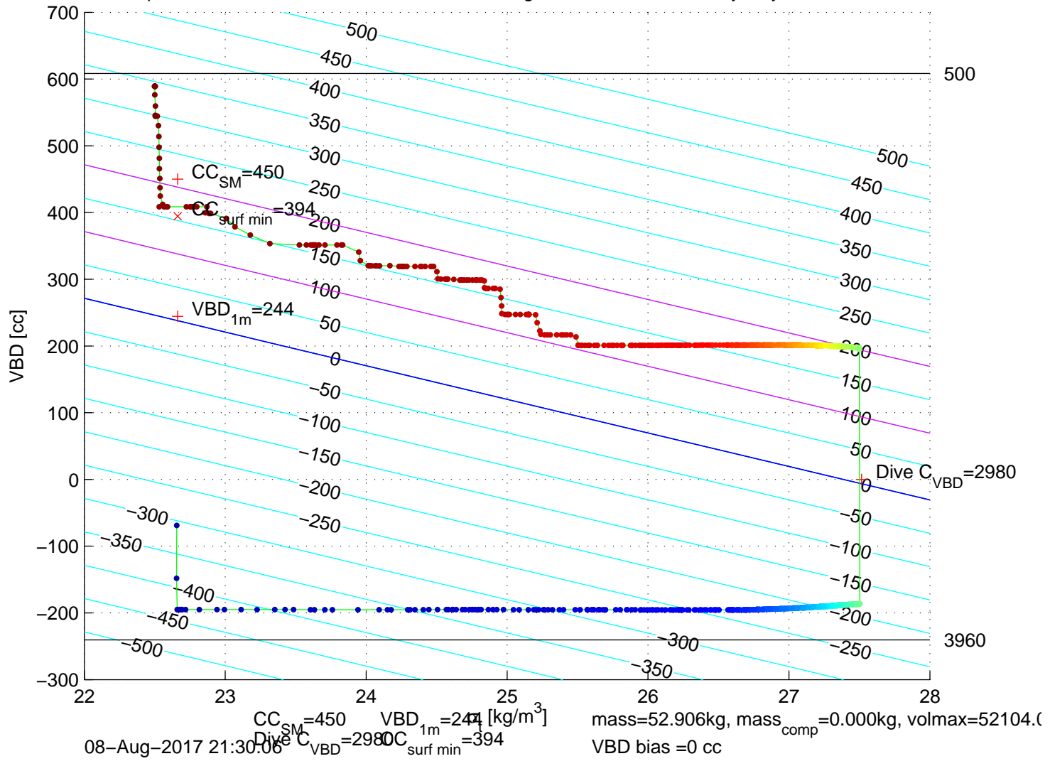
p6100162: SG610 Mission 7 Jul 2017 08–Aug–2017 20:55:54Z – buoyancy contoured
