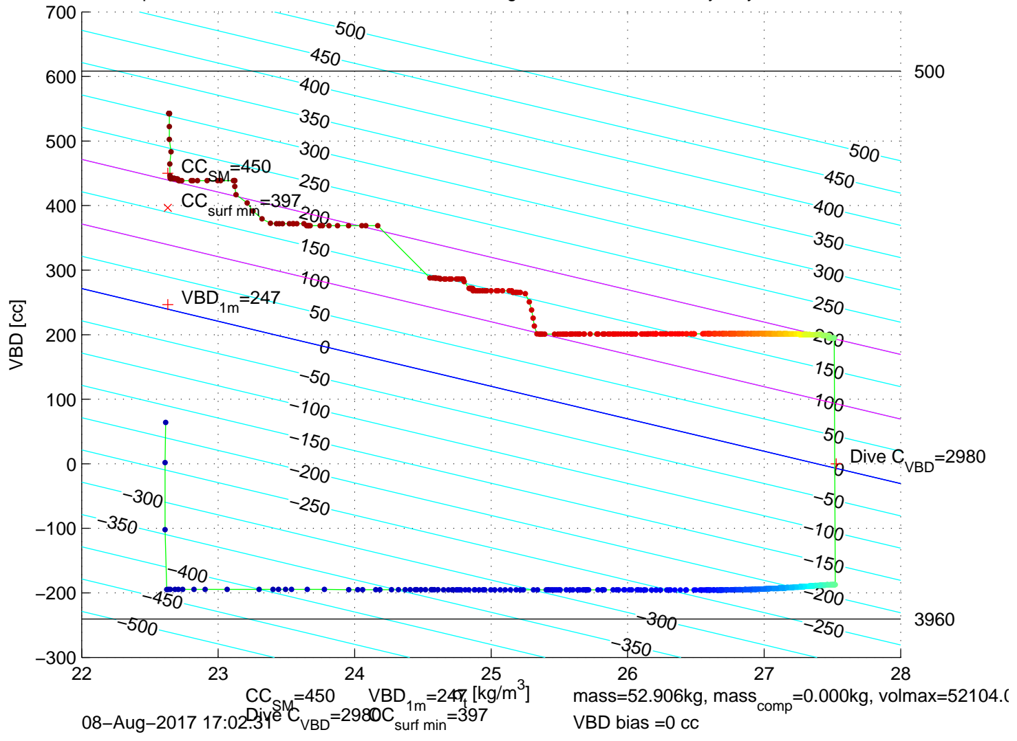
p6100161: SG610 Mission 7 Jul 2017 08–Aug–2017 16:27:22Z – buoyancy contoured
