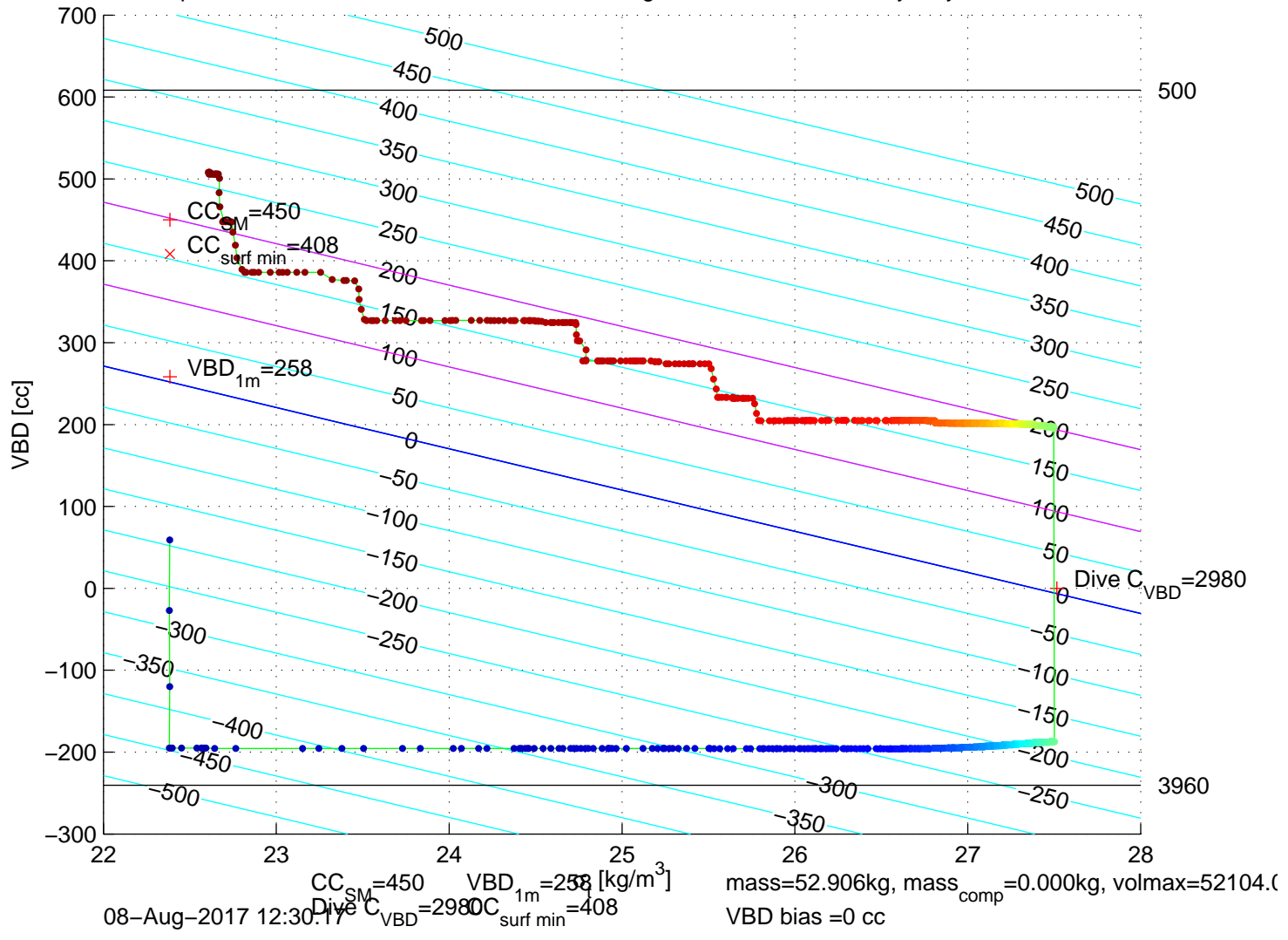
p6100160: SG610 Mission 7 Jul 2017 08–Aug–2017 12:09:56Z – buoyancy contoured
