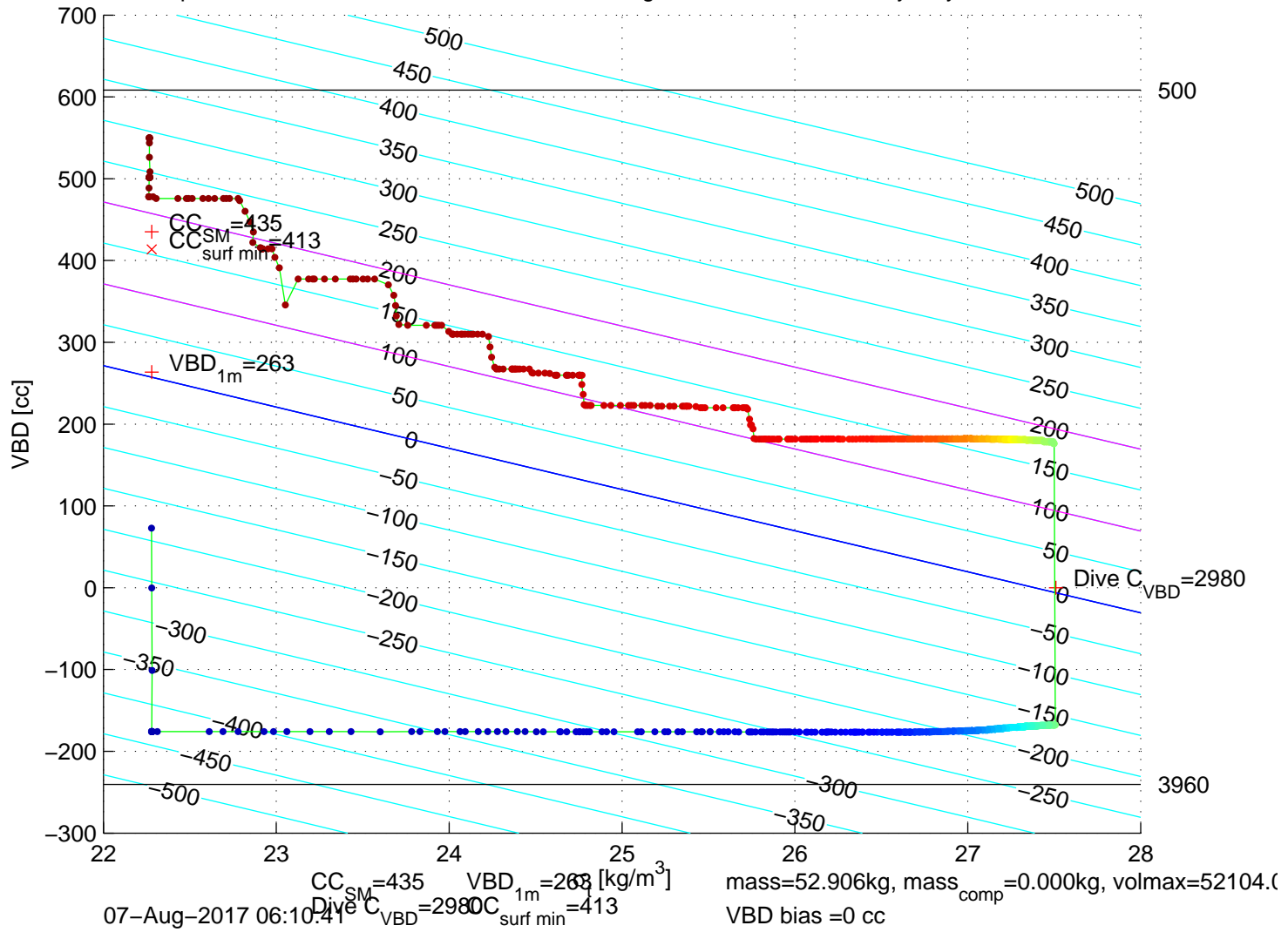
p6100153: SG610 Mission 7 Jul 2017 07–Aug–2017 05:36:22Z – buoyancy contoured
