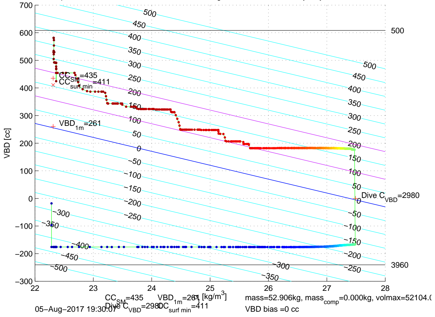
p6100145: SG610 Mission 7 Jul 2017 05–Aug–2017 19:02:06Z – buoyancy contoured
