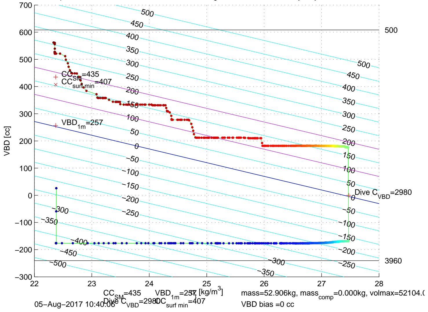
p6100143: SG610 Mission 7 Jul 2017 05–Aug–2017 10:16:52Z – buoyancy contoured
