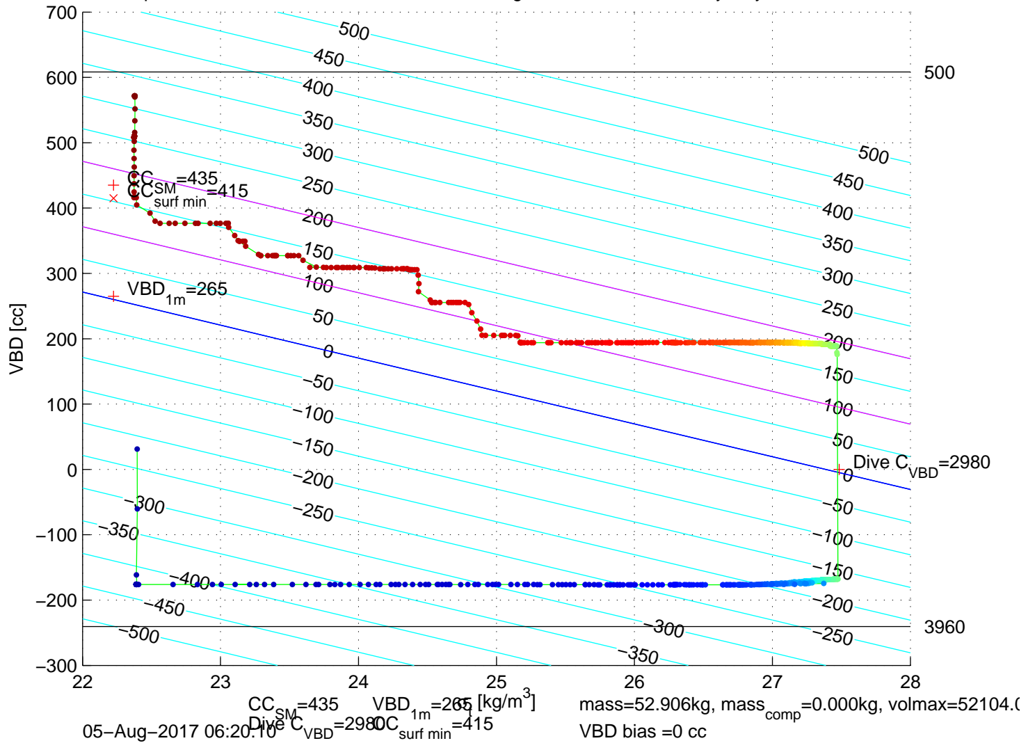
p6100142: SG610 Mission 7 Jul 2017 05–Aug–2017 06:03:37Z – buoyancy contoured
