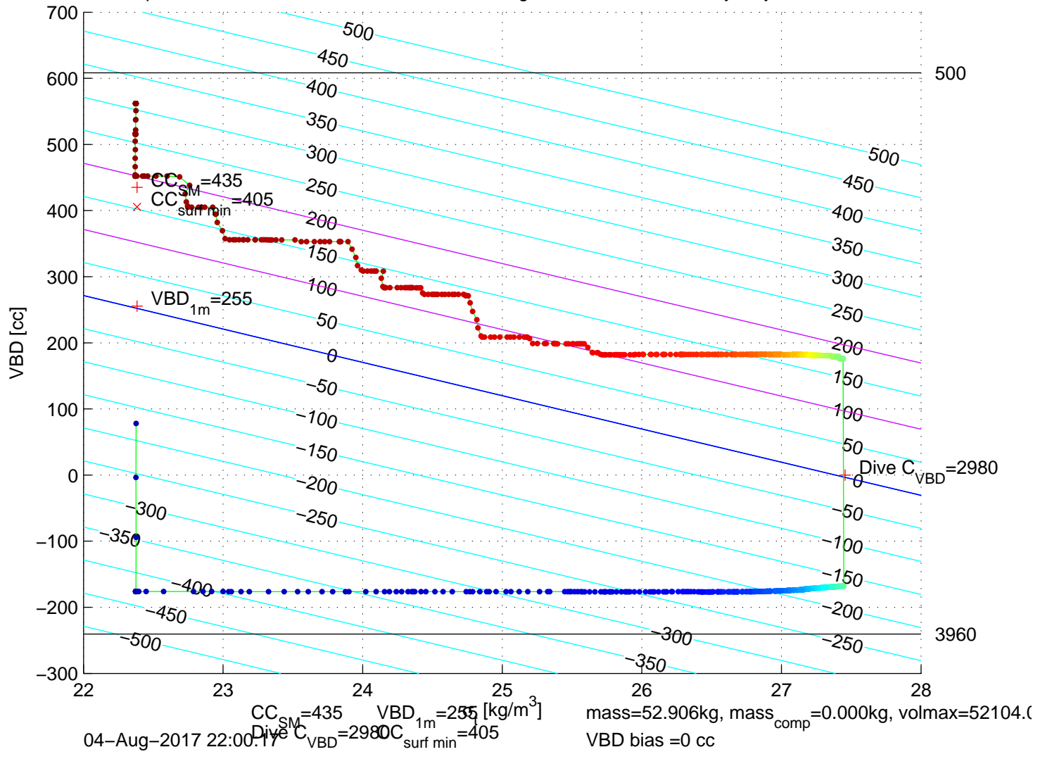
p6100140: SG610 Mission 7 Jul 2017 04–Aug–2017 21:31:39Z – buoyancy contoured
