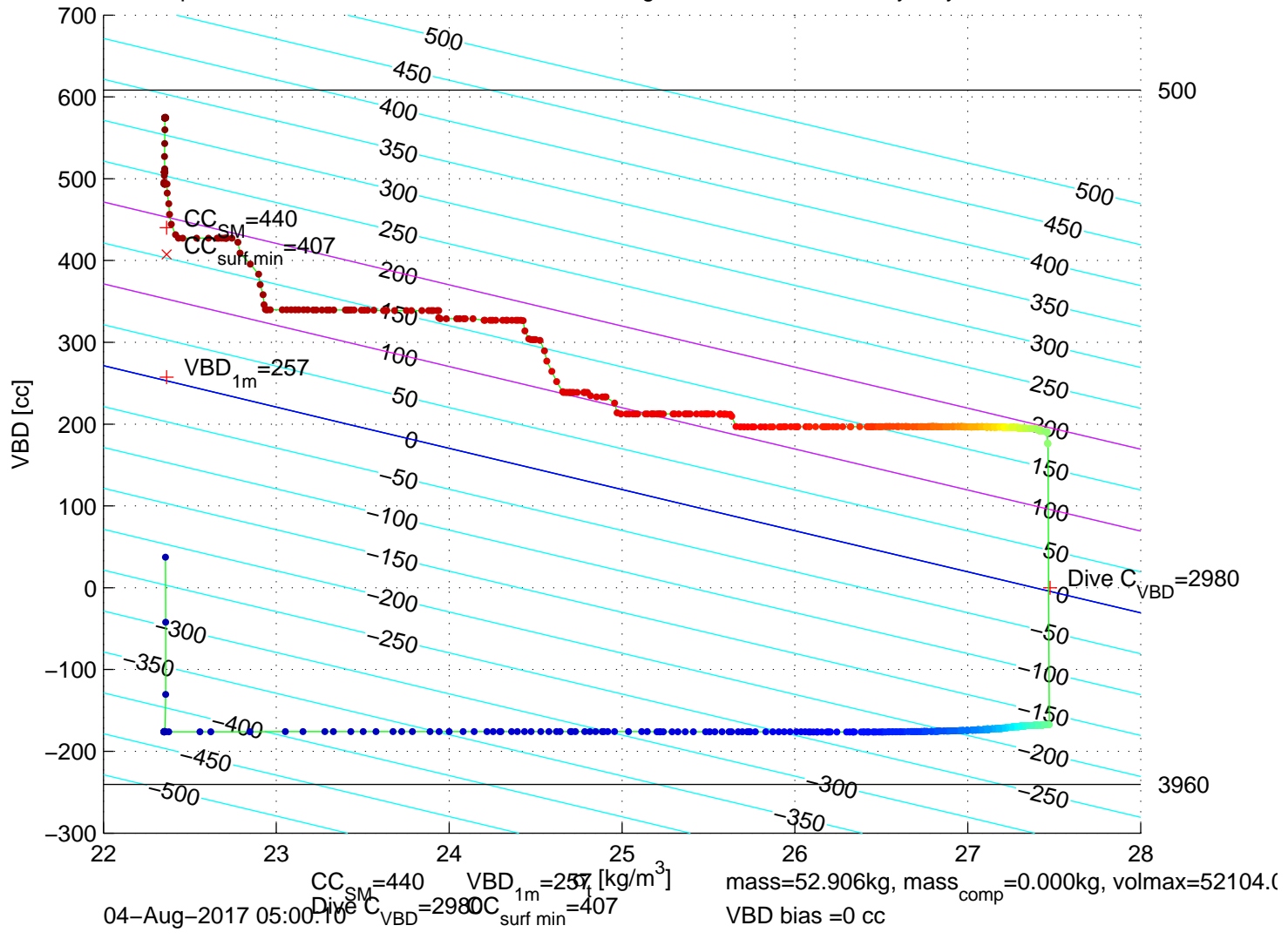
p6100136: SG610 Mission 7 Jul 2017 04–Aug–2017 04:38:25Z – buoyancy contoured
