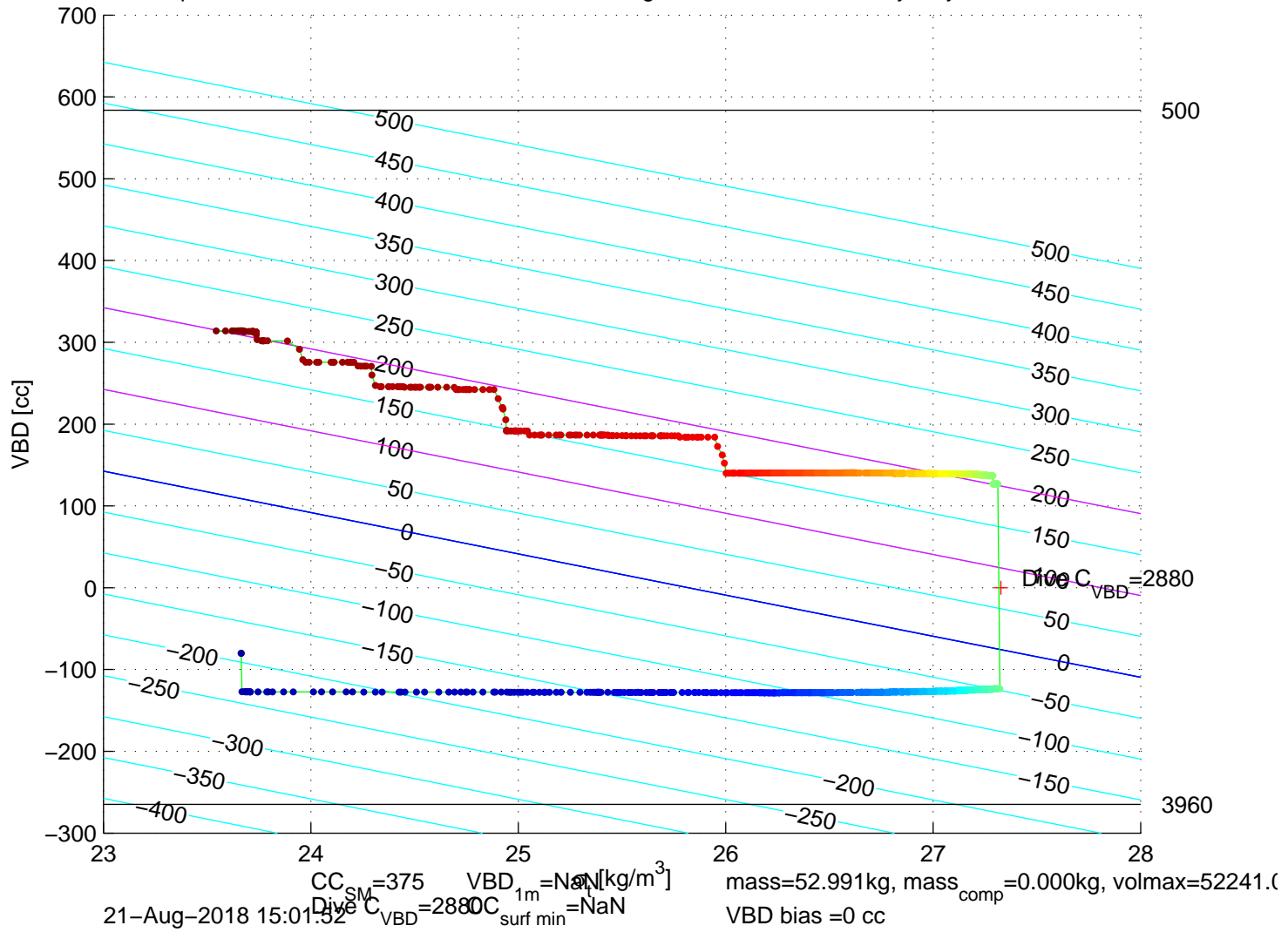
p6100114: SG610 Mission 8 Jul 2018 07–Aug–2018 14:06:43Z – buoyancy contoured
