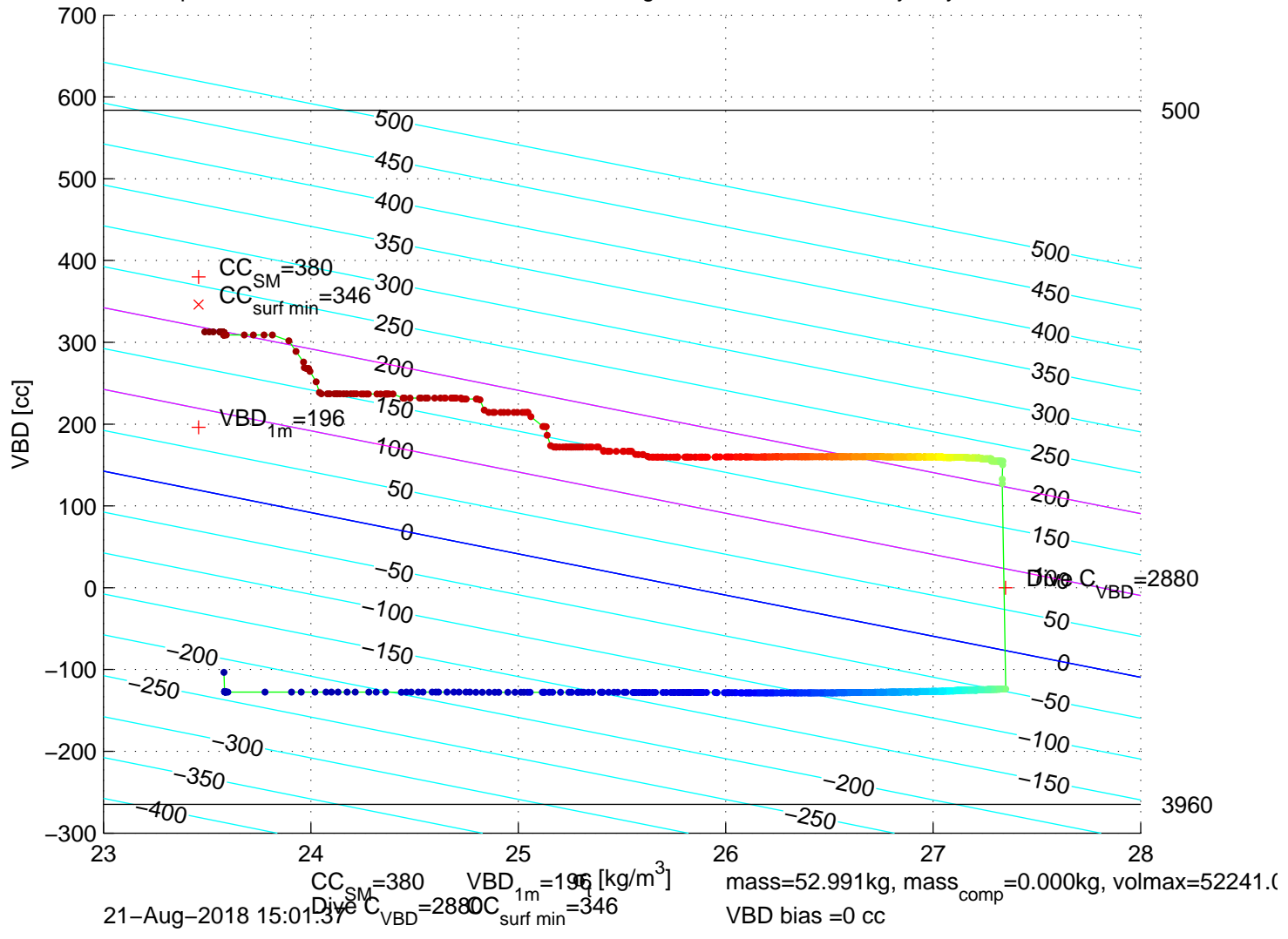
p6100103: SG610 Mission 8 Jul 2018 05–Aug–2018 14:02:32Z – buoyancy contoured
