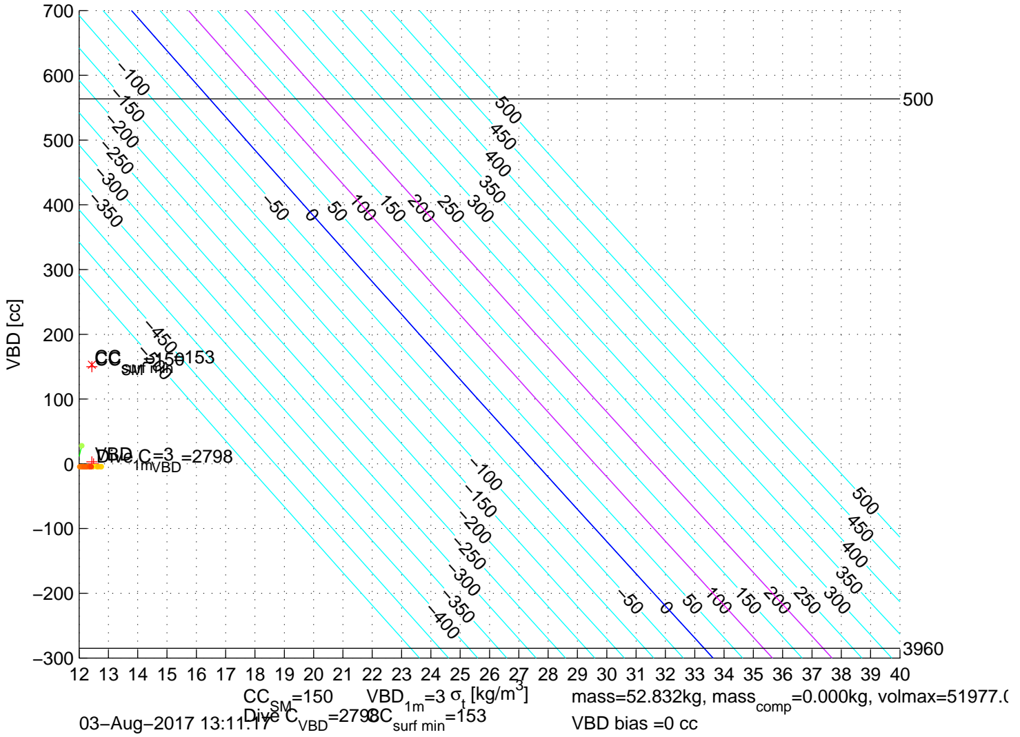
p6090035: SG609 Mission 7 Jul 2017 12-Jul-2017 12:32:51Z – buoyancy contoured
