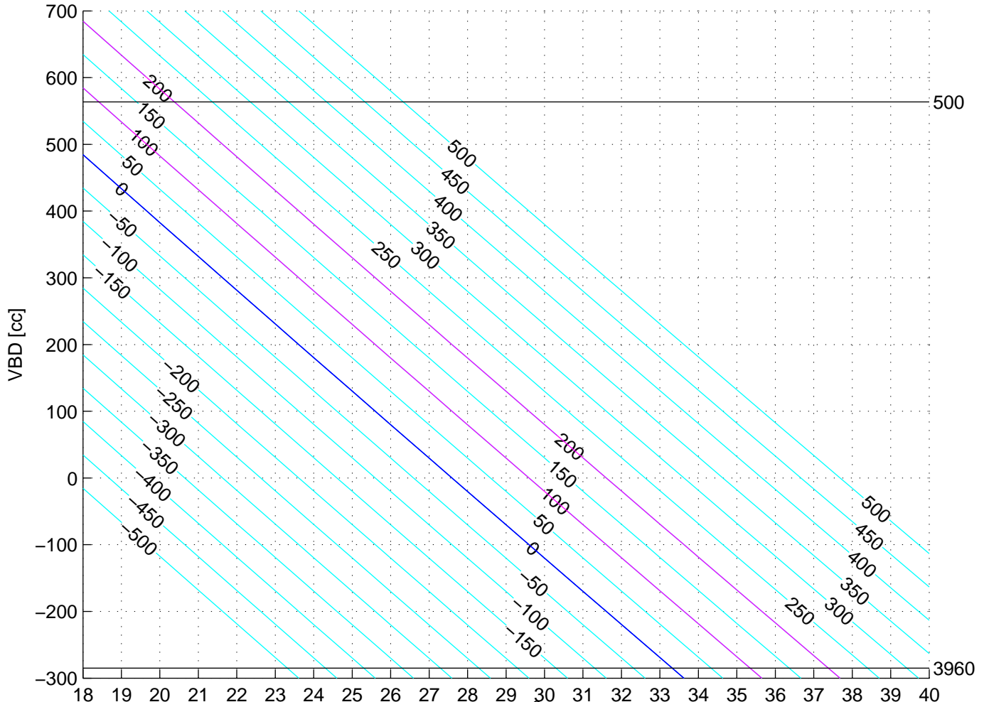
p6090034: SG609 Mission 7 Jul 2017 08-Aug-2017 15:42:03Z - buoyancy contoured
