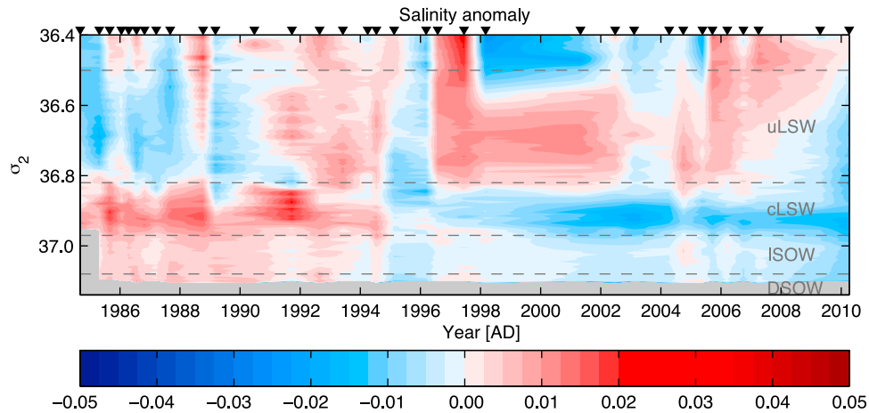
Figure 4. Hovmöller plot of the salinity anomaly obtained by averaging the salinity in the first 100 km offshore along \sigma_2 isopycnals in the DWBC at the Abaco line, with the water mass classification in dashed lines. The black triangles at the top indicate when the sections were occupied. It appears that on decadal timescales cLSW and the two types of overflow water become fresher, while uLSW becomes saltier.
