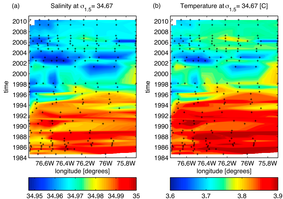
Figure 2. Hovmöller plots of (a) salinity and (b) temperature on the \sigma_{1.5} = 34.67 \text{ kg/m}^3 density surface (the core of the classical Labrador Sea Water) just off the Abaco coast. The black pluses indicate locations and timing of conductivity-temperature-depth (CTD) stations. Additional CTD stations outside of the domain shown here were used for the interpolation toward the domain boundaries. This figure is an extension of a similar figure (on approximately the same color scale) by Molinari et al. [1998] which showed that between 1994 and 1996 the core of the cLSW freshened and became colder. This extension shows that since then temperature and salinity have not come back to 1980s levels.
