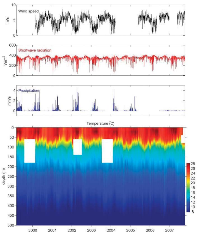
FIG. 2. PIRATA time series of atmospheric and oceanic properties at 0°, 23°W. Gaps indicate missing data due to instrument failure or vandalism.
