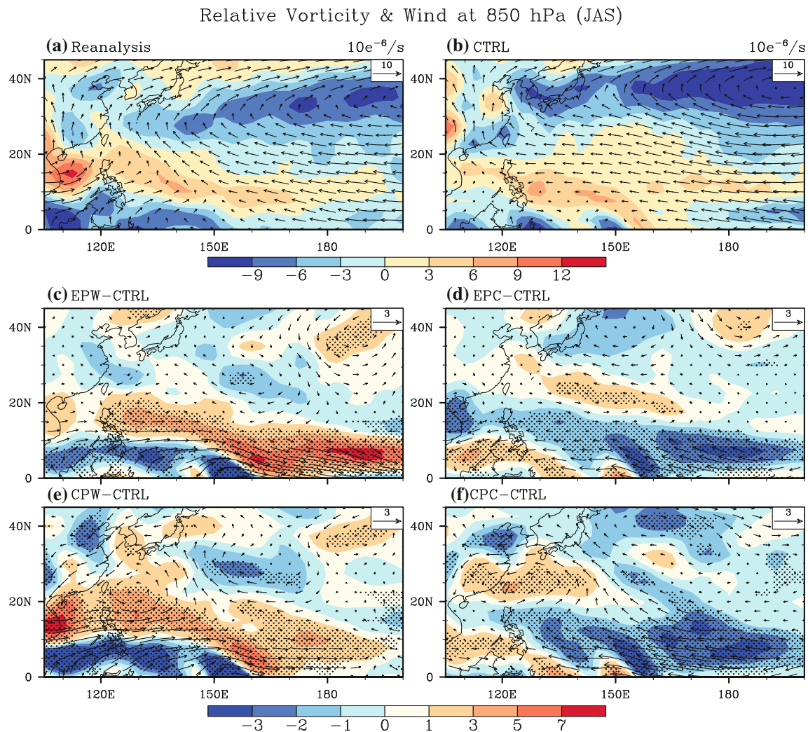
Fig. 2 The distribution of 850-hPa relative vorticity ( 10^{-6}/s ) and wind (m/s) during JAS in the WNP. Shown are the climatological means from a the NCEP–NCAR reanalysis and b the CTRL ensemble run. The differences between the EPW, EPC, CPW, and CPC runs and
