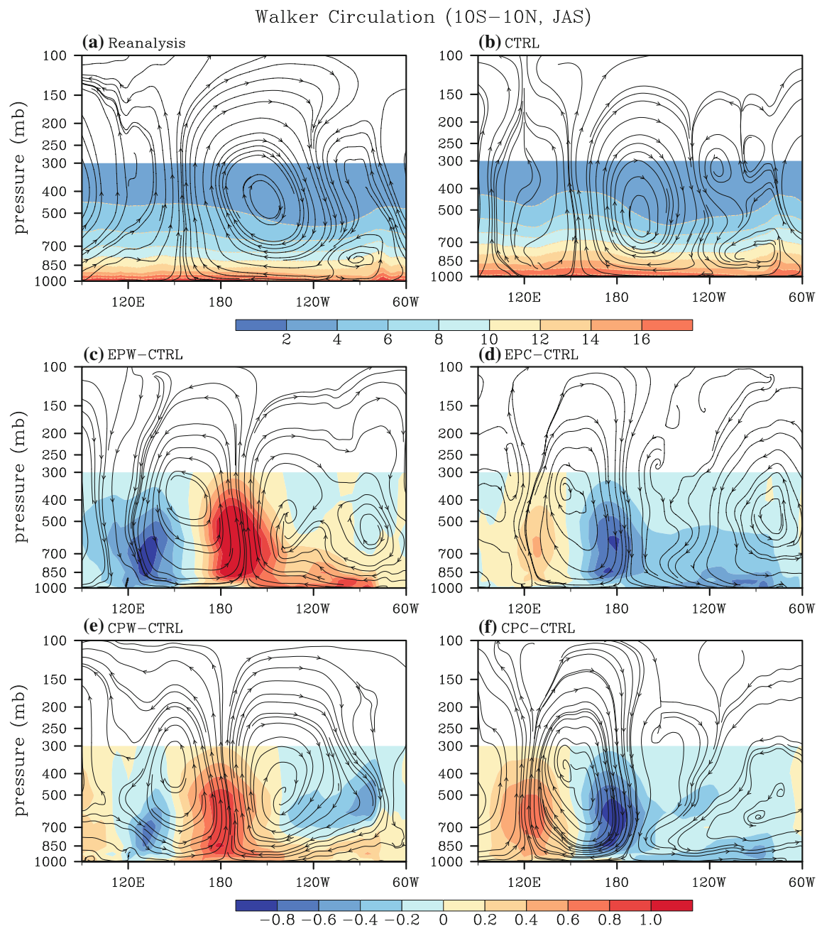
Fig. 10 The variations of the Walker circulation and specific humidity ( shading ; g/kg) during JAS. The Walker circulation is calculated by averaging divergent wind and vertical velocity between 10°S and 10°N. Shown are the climatological means from a the
