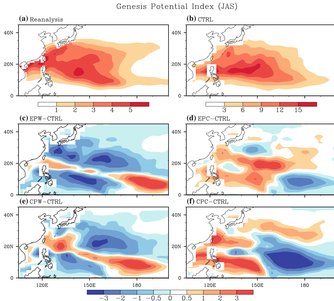
Fig. 6 The distribution of GPI during JAS in the WNP. Shown are the climatological means from a the NCEP–NCAR reanalysis and b the CTRL ensemble run. The differences between the EPW, EPC, CPW, and CPC runs and the CTRL run are shown in c , d , e , and f , respectively
