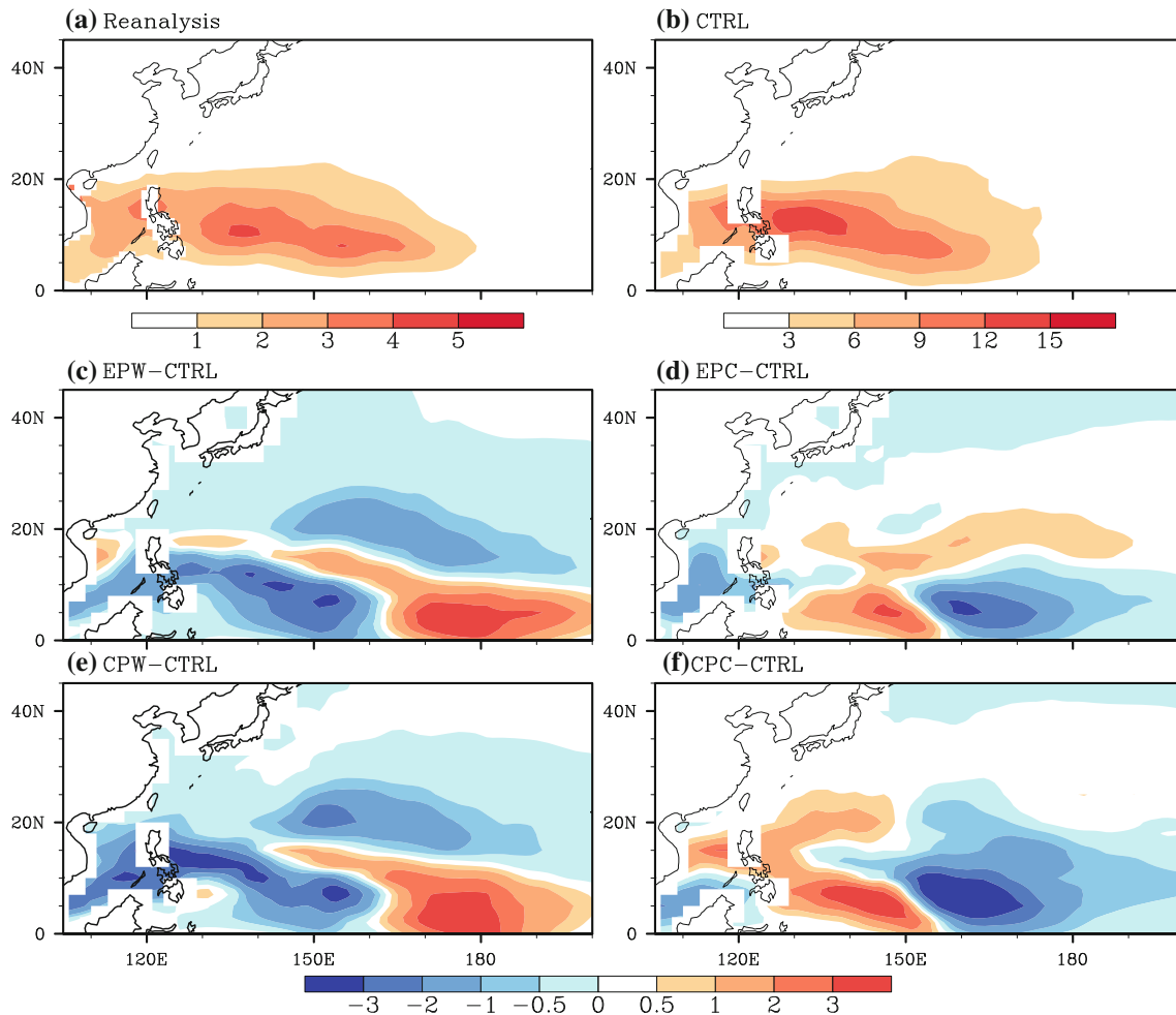
Fig. 7 The distribution of GPI during OND in the WNP. Shown are the climatological means from a the NCEP–NCAR reanalysis and b the CTRL ensemble run. The differences between the EPW, EPC, CPW, and CPC runs and the CTRL run are shown in c , d , e , and f , respectively
