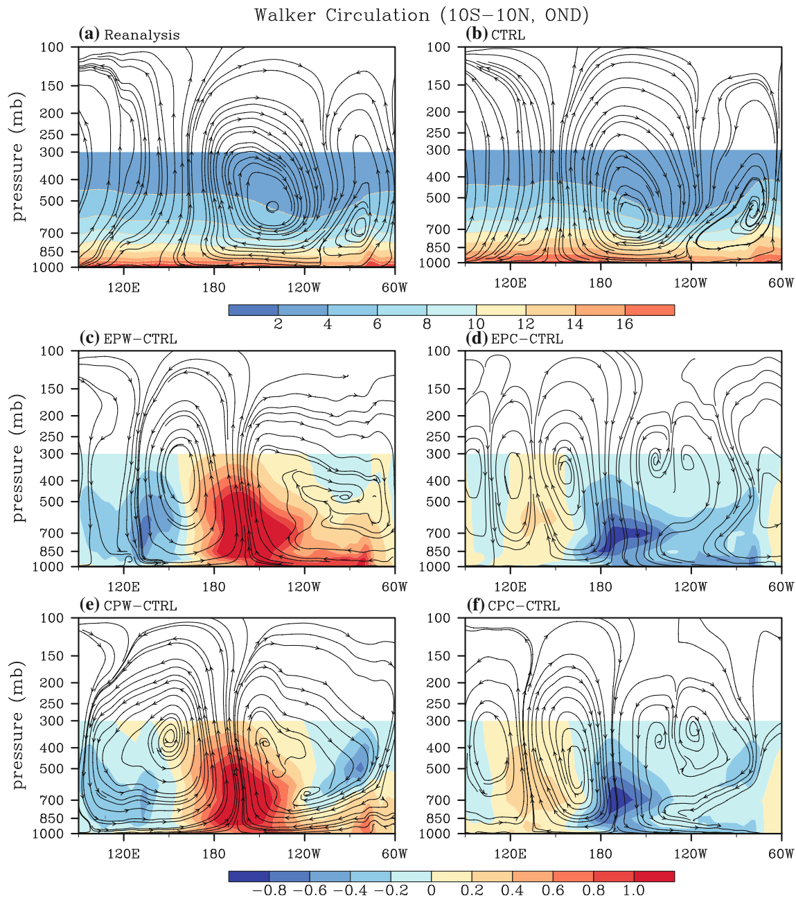
Fig. 11 The variations of the Walker circulation and specific humidity ( shading ; g/kg) during OND. The Walker circulation is calculated by averaging divergent wind and vertical velocity between 10°S and 10°N. Shown are the climatological means from a the
