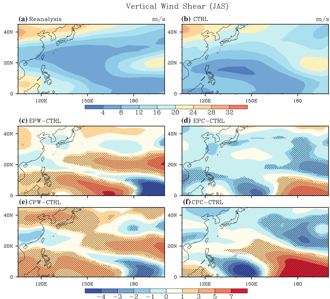
Fig. 4 The distribution of VWS (m/s) during JAS in the WNP. Shown are the climatological means from a the NCEP–NCAR reanalysis and b the CTRL ensemble run. The differences between the
