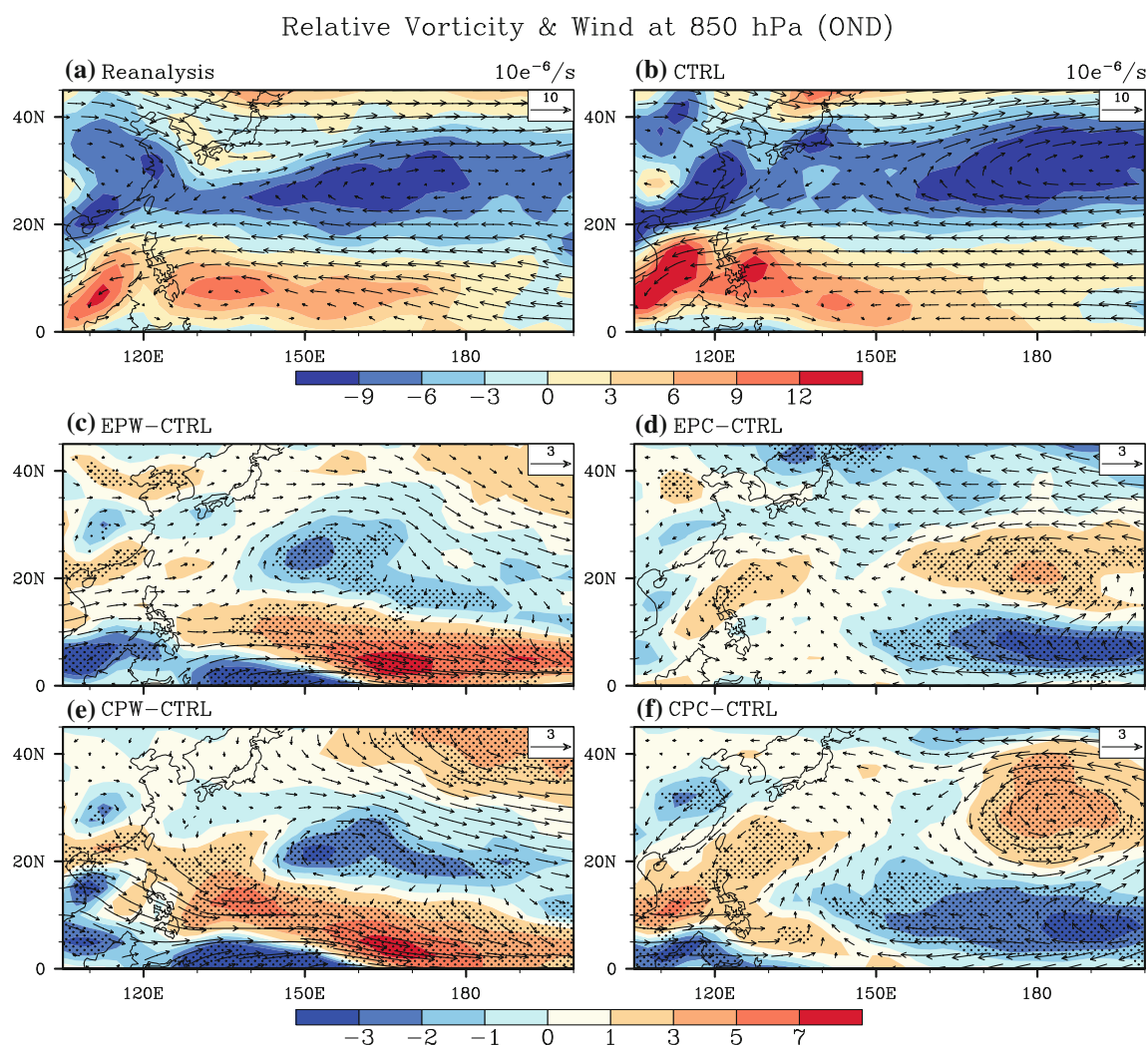
Fig. 3 The distribution of 850-hPa relative vorticity ( 10^{-6}/s ) and wind (m/s) during OND in the WNP. Shown are the climatological means from a the NCEP–NCAR reanalysis and b the CTRL ensemble run. The differences between the EPW, EPC, CPW, and CPC runs and
