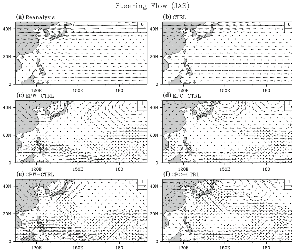
Fig. 8 The distribution of the TC steering flow (m/s) during JAS in the WNP. Shown are the climatological means from a the NCEP–NCAR reanalysis and b the CTRL ensemble run. The differences
