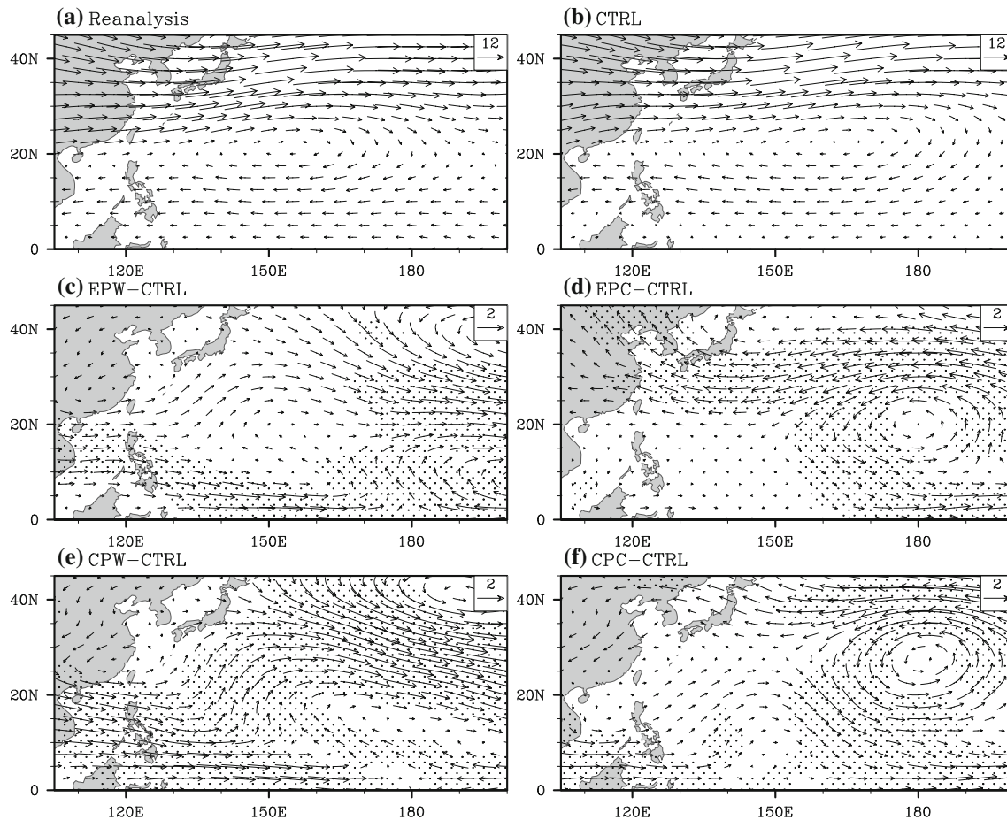
Fig. 9 The distribution of the TC steering flow (m/s) during OND in the WNP. Shown are the climatological means from a the NCEP–NCAR reanalysis and b the CTRL ensemble run. The differences
