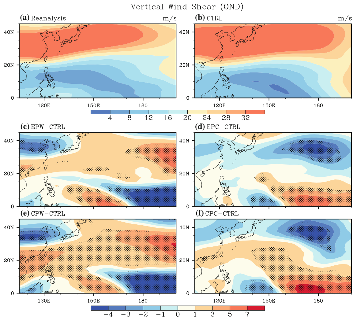
Fig. 5 The distribution of VWS (m/s) during OND in the WNP. Shown are the climatological means from a the NCEP–NCAR reanalysis and b the CTRL ensemble run. The differences between the
