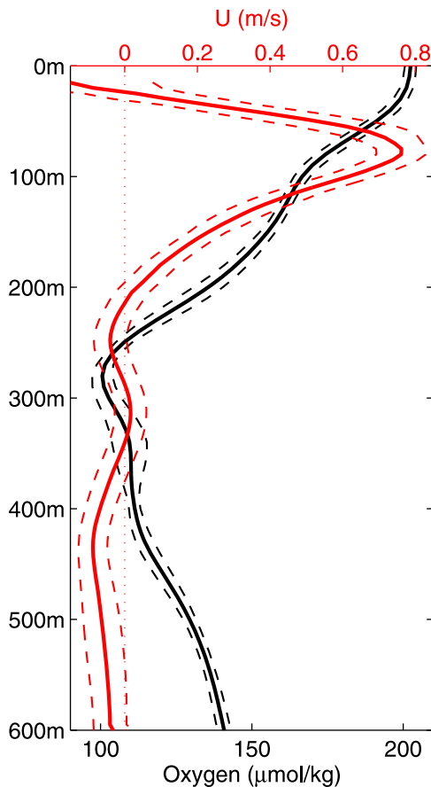
Figure 4. Mean equatorial profiles of observed zonal velocity (red, top axis) and oxygen (black, bottom axis) at 23°W, with standard error of the mean (dashed). The zonal velocity profile was obtained from more than seven years of moored observations (Figure 5). The oxygen profile is taken from the mean shipboard section (Figure 2b). The red dotted line marks zero velocity.
