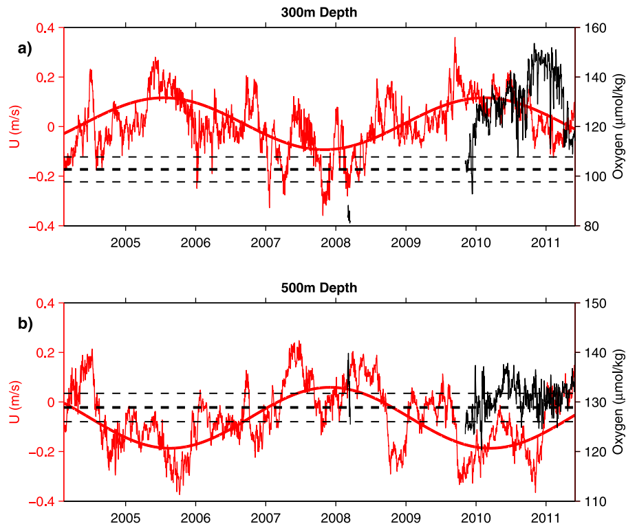
Figure 6. Zonal velocity from moored observations at the equator, 23°W, with overlaid 1670-d harmonic fit (red, left axis) and oxygen concentration from moored instruments (black, right axis) at (a) 300 m and (b) 500 m depth. The mean oxygen concentration at 300 m and 500 m depth from ship sections is 103 \pm 5 \mu\text{mol kg}^{-1} and 129 \pm 3 \mu\text{mol kg}^{-1} (thick black dashed lines), respectively, with standard errors marked by thin black dashed lines. Note that the oxygen range in Figure 6a is twice as large as in Figure 6b.
