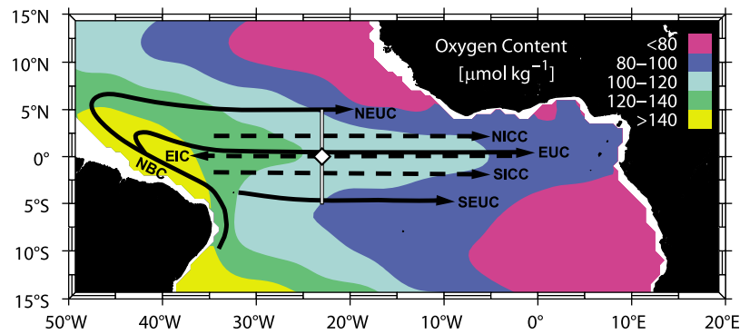
Figure 1. Climatological distribution of the oxygen concentration [ \mu\text{mol kg}^{-1} ] at 300–500 m in the tropical Atlantic [Gouretski and Koltermann, 2004], with superimposed repeat ship section along the 23°W meridian (thick white line) and the equatorial mooring position (diamond). Also included are major thermocline (black solid arrows) and intermediate (black dashed arrows) current branches: North Brazil Current (NBC), North and South Equatorial Undercurrent (NEUC, SEUC), and Equatorial Undercurrent (EUC), as well as Southern and Northern Intermediate Countercurrents (NICC, SICC), and Equatorial Intermediate Current (EIC).
