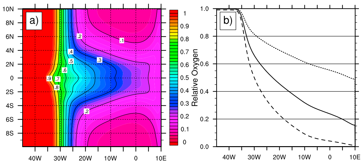
Figure 10. (a) Horizontal map and (b) equatorial distribution of the simulated mean relative oxygen concentration averaged over a full basin-mode cycle. Note that oxygen is normalized relative to the value used for the restoring at the western boundary. In Figure 10b, simulations with the oxygen consumption coefficient increased (dashed)/decreased (dotted) by a factor of five are also included.
