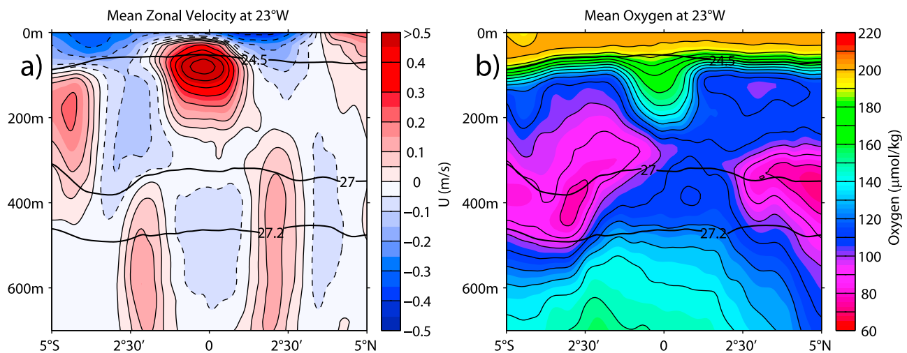
Figure 2. Mean (a) zonal velocity and (b) oxygen concentration along 23°W from ship sections (update from Brandt et al. [2010]). Thick black solid lines mark surfaces of uniform potential density. In Figure 2a, negative values indicating westward flow are shown by dashed contours and the contour interval is 5 \text{ cm s}^{-1} within the range from -10 \text{ cm s}^{-1} to 10 \text{ cm s}^{-1} and 10 \text{ cm s}^{-1} elsewhere.
