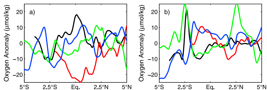
Figure 8. Observed meridional oxygen structure along 23°W. Shipboard measurements taken during research cruises in June 2006 (black), February/March 2008 (red), November 2009 (green), and May/June 2011 (blue) were averaged (a) between 280 and 380 m depth and (b) between 450 and 550 m depth.
