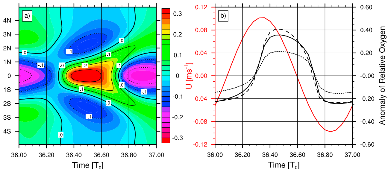
Figure 11. Simulated anomaly of relative oxygen at 23^\circ\text{W} for a full basin mode cycle, T_0 = 1670 d, (a) as a function of latitude and time (in parts of the cycle) and (b) only at the equator (black, right axis). The zonal velocity used to force the advection-diffusion model is included in Figure 11b (red, left axis). The simulation started after a model spin-up of 36 basin-mode cycles to ensure a steady, oscillating oxygen distribution. In Figure 11a, negative values are shown by dashed contours and the contour interval is 0.1. In Figure 11b, simulations with the oxygen consumption coefficient increased (dashed)/decreased (dotted) by a factor of five are also included.
