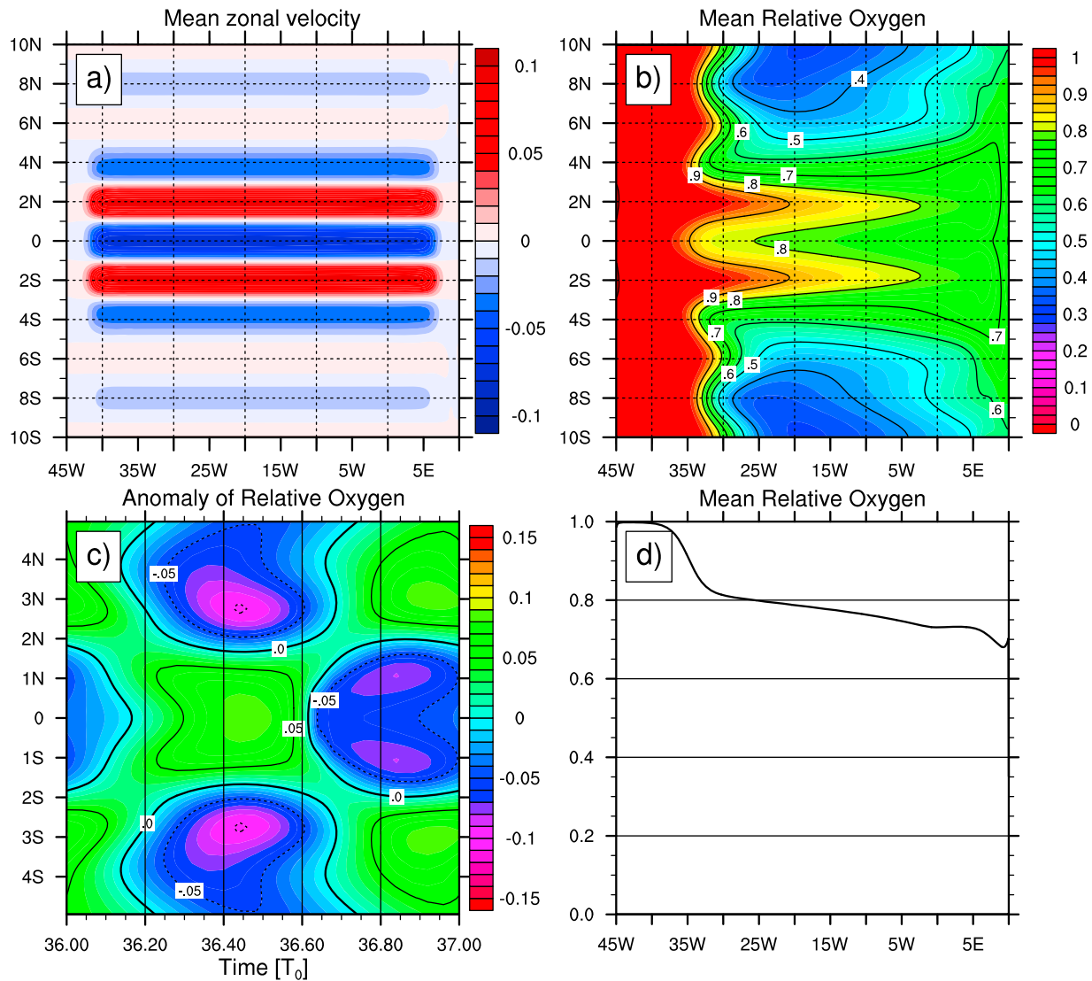
Figure 14. Same as Figure 13, but the mean zonal velocity field used in this simulation corresponds to the observed zonal velocity at 500 m depth (cf. Figure 3c).
