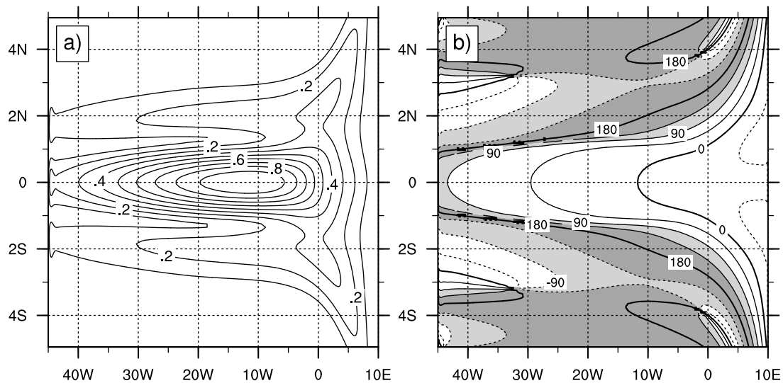
Figure 9. (a) Amplitude and (b) phase of the zonal velocity associated with an equatorial basin mode for a high-order baroclinic mode (gravity wave speed c = 0.17 \text{ m s}^{-1} ) using a lateral eddy viscosity of 200 \text{ m}^2 \text{ s}^{-1} as simulated by the reduced-gravity model of Greatbatch et al. [2012] after subtracting the divergent part of the velocity field (see the text for details). The amplitude is normalized by the maximum zonal velocity amplitude. In Figure 9b, solid contours show positive phase, indicating a lag compared to zero, and dashed contours show negative phase. The contour interval is 45^\circ .
