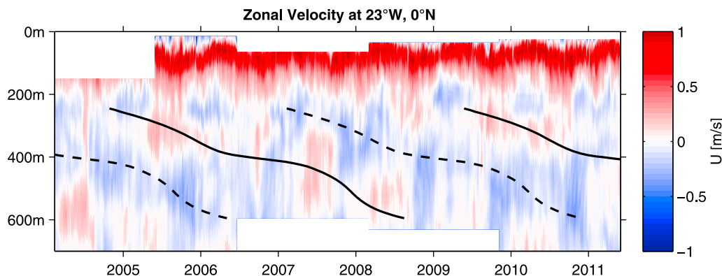
Figure 5. Zonal velocity from moored observations at the equator, 23°W, with superimposed phase lines obtained from a harmonic analysis using a period of 1670 days (solid: maximum eastward velocity, dashed: maximum westward velocity).
