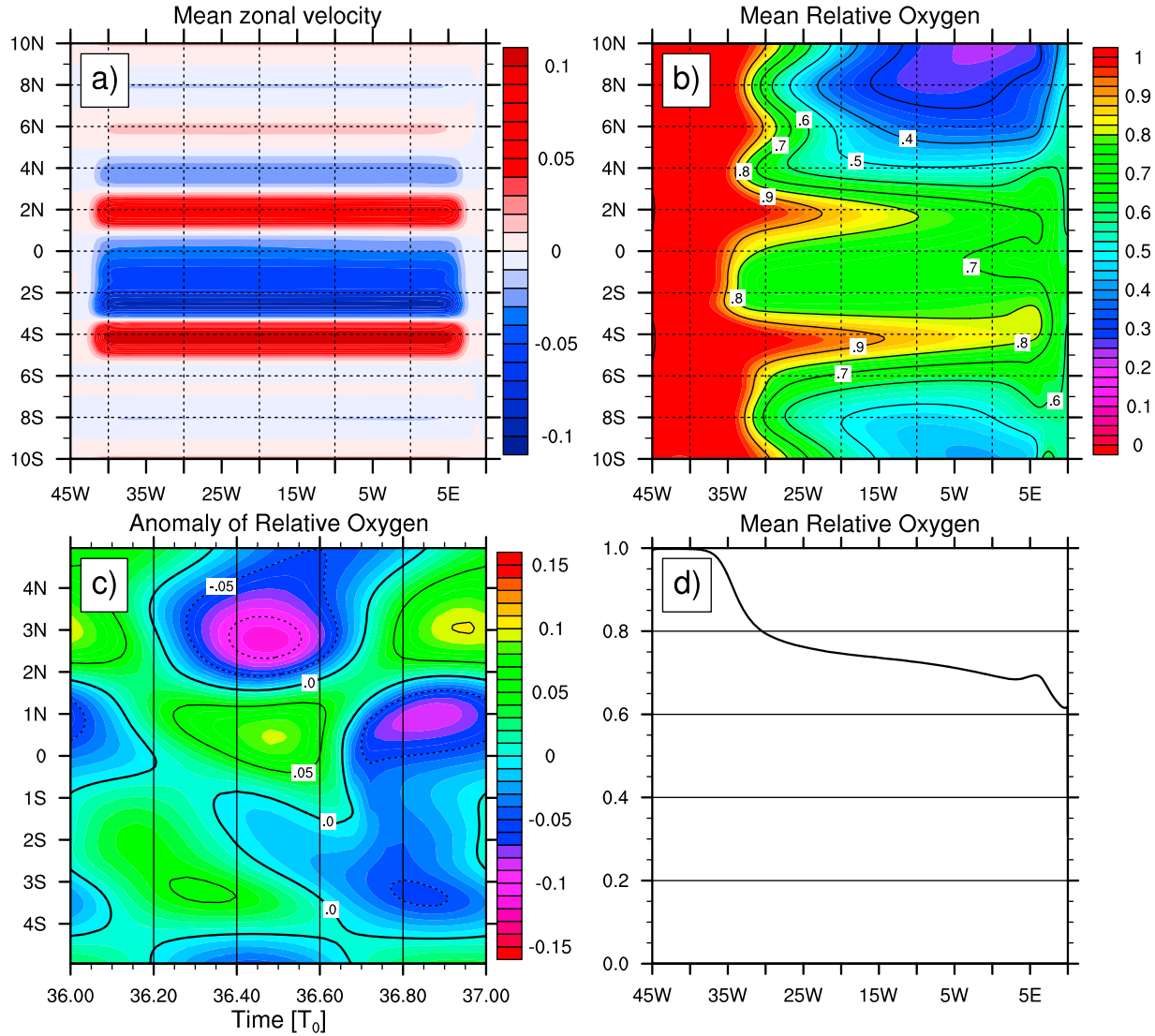
Figure 13. Horizontal maps of (a) the prescribed mean zonal velocity and (b) the simulated mean relative oxygen concentration averaged over a full basin-mode cycle. (c) The simulated anomaly of relative oxygen at 23^\circ\text{W} for a full basin-mode cycle, T_0 = 1670 d, as a function of latitude and time (in parts of the cycle). (d) The equatorial distribution of the simulated mean relative oxygen concentration averaged over a full basin-mode cycle. The mean zonal velocity field used in this simulation corresponds to the observed zonal velocity at 300 m depth (cf. Figure 3b).
