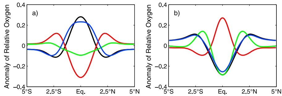
Figure 12. Simulated meridional oxygen structure along 23^{\circ}\text{W} . Simulations are extracted corresponding to the measurements shown in Figure 8 in the depth interval 280 to 380 m (a) at 263 days (black), 884 days (red), 1505 days (green), and 403 days (blue) and in the depth interval 450 to 550 m (b) at 1136 days (black), 87 days (red), 708 days (green), and 1276 days (blue) after maximum eastward velocity of the basin-mode cycle at the equator, 23^{\circ}\text{W} .
