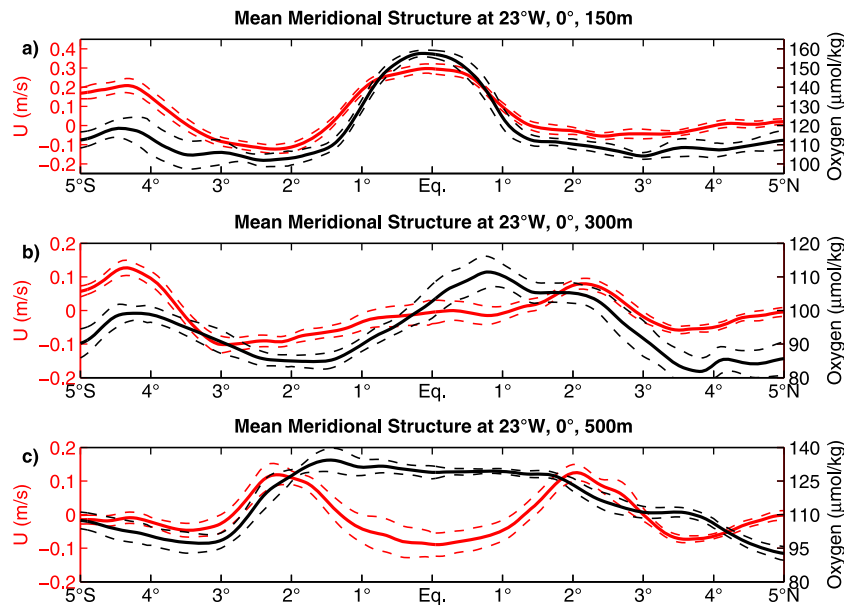
Figure 3. Mean meridional structure of observed zonal velocity (red, left axis) and oxygen (black, right axis) along 23°W at (a) 150 m, (b) 300 m, and (c) 500 m, with standard errors of the mean (dashed).
