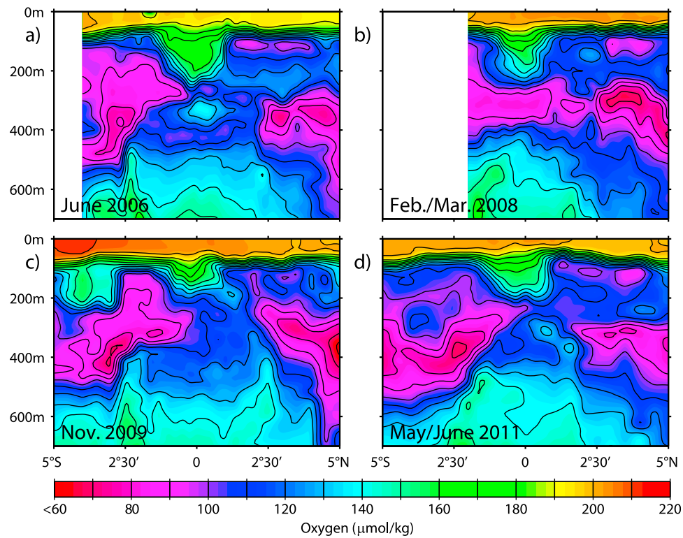
Figure 7. Oxygen distributions along 23°W taken during research cruises in (a) June 2006, (b) February/March 2008, (c) November 2009, and (d) May/June 2011.
