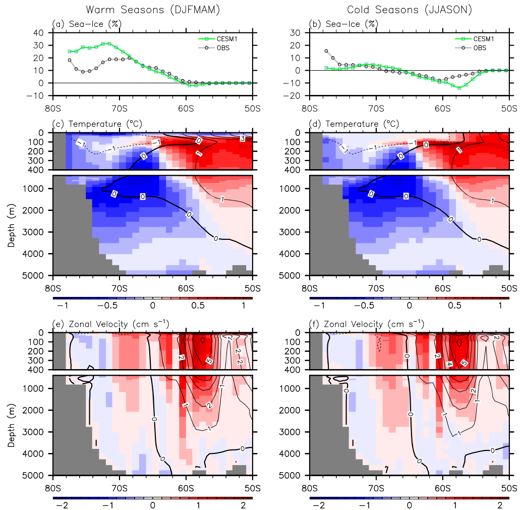
Figure 8. Linear trends of (a, b) Antarctic sea-ice concentration, (c, d) ocean temperatures, and (e, f) zonal velocity averaged over the Atlantic sector (60°W–0°) for (a, c, e) the warm and (b, d, e) cold seasons over the period of 1985–2014, obtained from the historical simulation. Observed linear trends of Antarctic sea-ice concentration over the period of 1979–2014 averaged over the Atlantic sector are also shown in Figures 8a and 8b. The black lines in Figures 8c, 8d, 8e, and 8f indicate the climatological temperatures and zonal velocity, respectively. The units are % in 35 years for sea-ice concentration, °C in 35 years for ocean temperature, and 10^{-2} \text{ m s}^{-1} in 35 years for zonal velocity.
