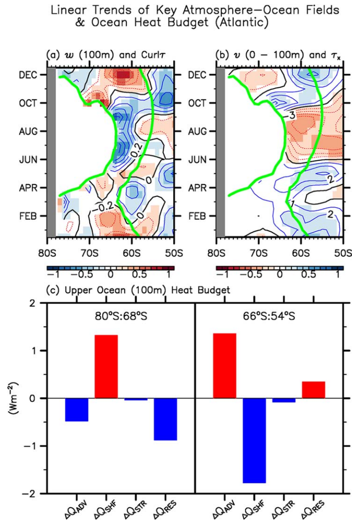
Figure 9. As in Figure 5, but for the Atlantic sector ( 60^{\circ}\text{W} – 0^{\circ} ) and (c) averaged over (left) the 80^{\circ}\text{S} – 68^{\circ}\text{S} and (right) 66^{\circ}\text{S} – 54^{\circ}\text{S} latitude bands over the Atlantic sector.
