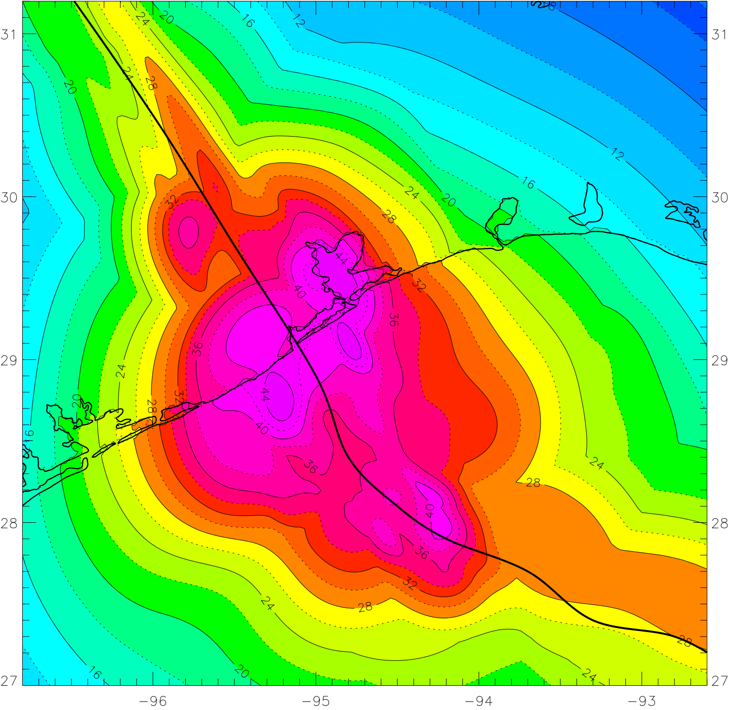
ALICIA: MAXIMUM WIND CONTOURS (M/S)
