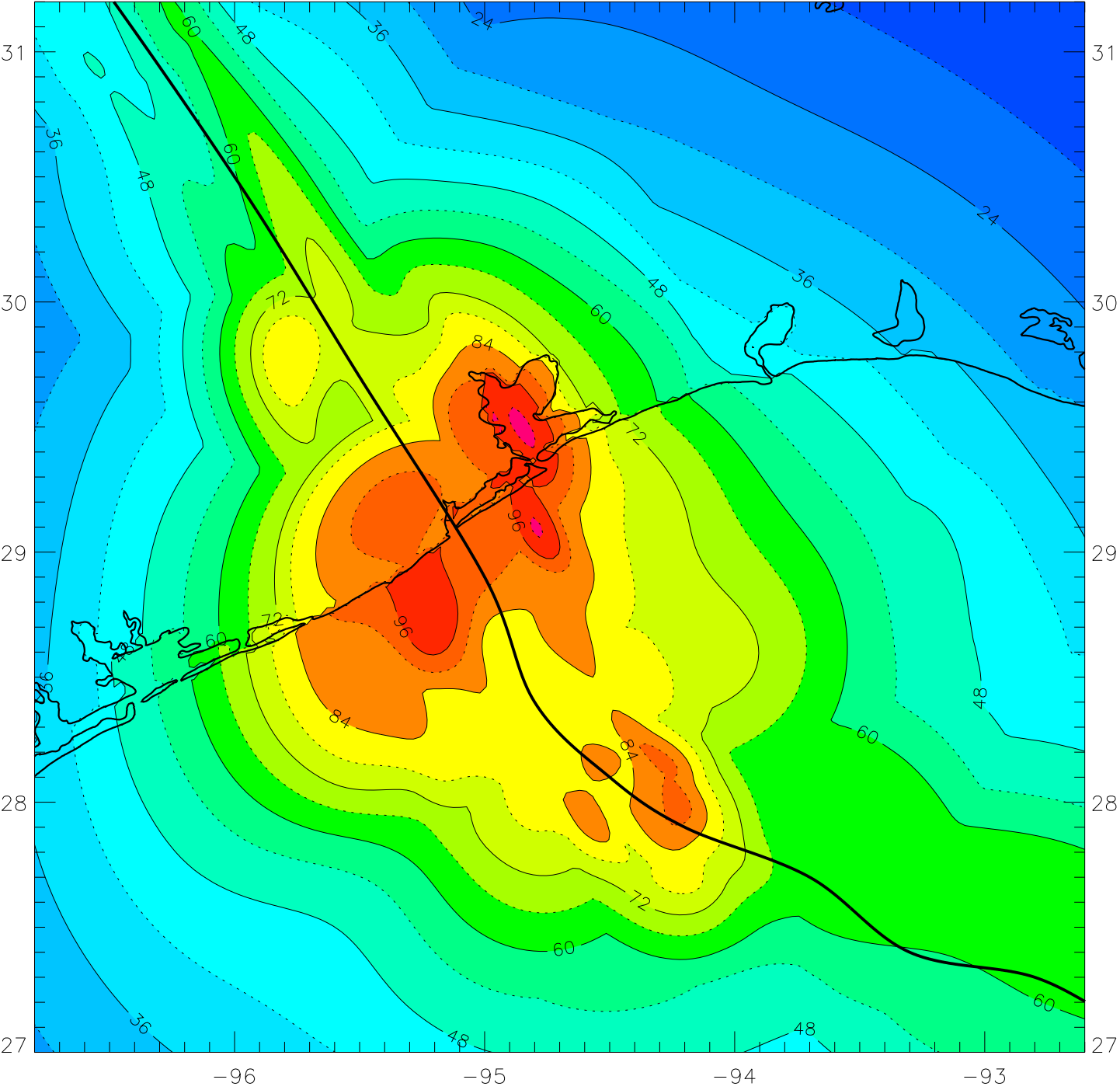
ALICIA: MAXIMUM WIND CONTOURS (MPH)
