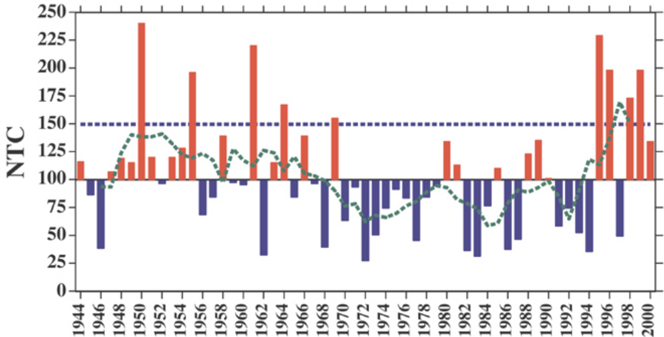
Supplemental Figure 2. Net Tropical Cyclone activity (NTC) in the North Atlantic hurricane basin for 1944-2000. Values above (>100%) and below (<100%) average activity are shown as solid red and blue columns, respectively. Dashed (green) curved line is 5-year running mean. Also shown is the threshold value (150%) for hyperactive years (dashed blue straight line). NTC gives a measure of the overall activity in a season by combining information on frequency, intensity and duration. By definition, NTC tends to be weighted somewhat towards the stronger systems. NTC \equiv (\%TS + \%H + \%MH + \%TSD + \%HD + \%MHD) / 6 , where TS, H, and MH are the number of systems reaching (at least) tropical storm, hurricane and major hurricane status, respectively, TSD, HD and MHD are the cumulative durations (summed for 6-hr intervals) at each status for all storms in a particular season, and “%” for each parameter is the percentage of the 1950 to 1990 climatological mean attained in that season (4). If all of the parameters are near their respective long-term means, NTC would be ~100%, i.e., an “average” season. Since 1944, values for NTC have ranged from a minimum of 28% (1972) to a high of 243% (1950). The mean NTC for the years 1971-1994 is only 76% compared with a mean of 114% for 1944-1970 (Supplemental Table 1). Six years (out of 25) during 1971-1994 had above-average activity (i.e., >100%) compared with 15 (out of 26) in the earlier period. Five of the years during 1944-1970 were “hyperactive” (defined as NTC \geq 150\% ) while there were no hyperactive years during 1971-1994. The hyperactive year 1995 marked the first since 1969. The mean NTC for 1995-2000 was 165% with four of the years hyperactive. In 2000, during which neutral ENSO conditions prevailed, the season still produced well-above-average activity.
