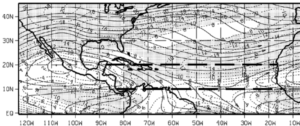
Supplemental Figure 1. Climatological winds from the NCEP/NCAR Reanalysis (9) for 1948-2000 averaged for August-September-October (ASO). Streamlines and isotachs ( \text{m s}^{-1} ) are shown.
