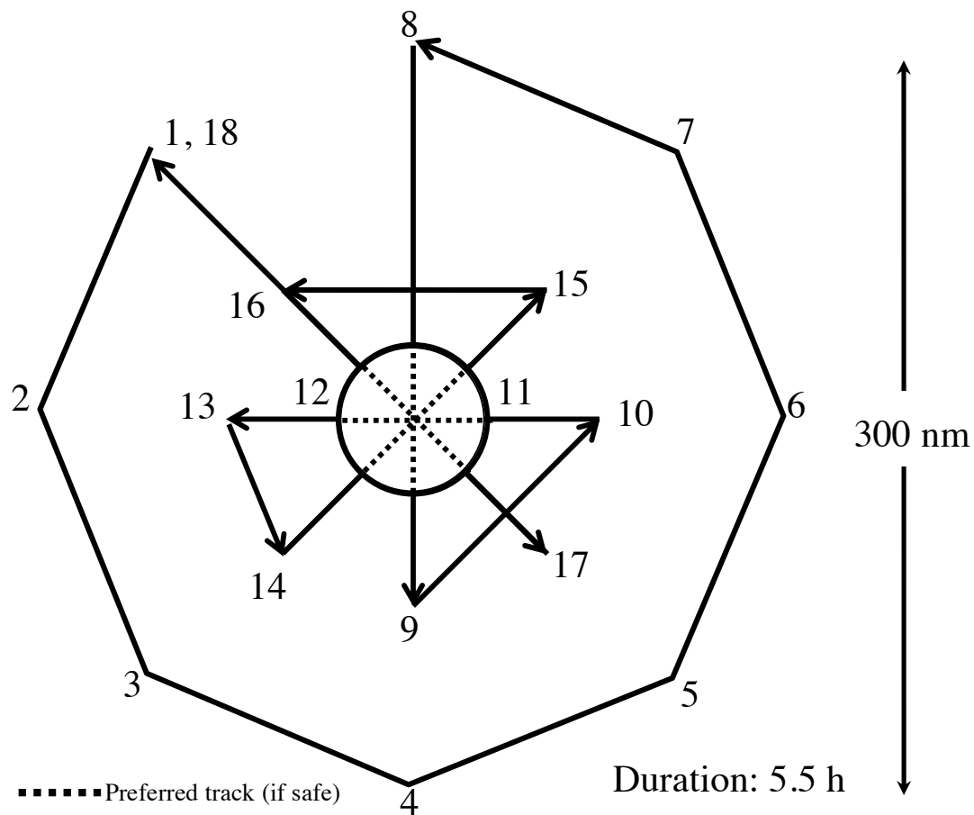
Figure 2-6: G-IV tail Doppler radar pattern – Surveillance/TDR combination
