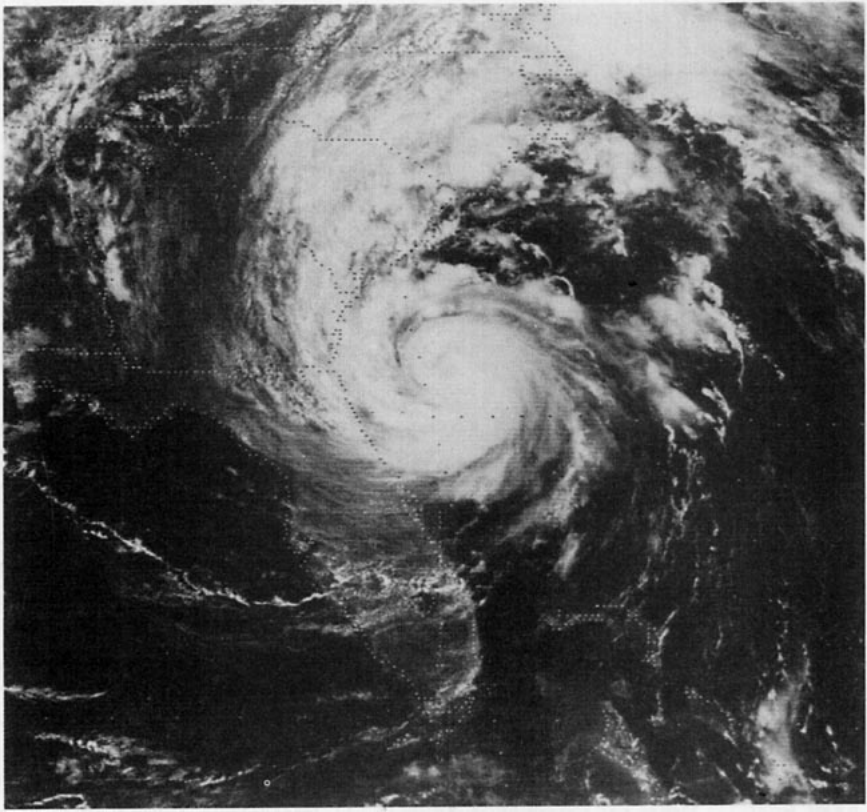
FIG. 4. GOES-West visible satellite picture of Hurricane Diana at 1700 GMT 10 September 1984.
