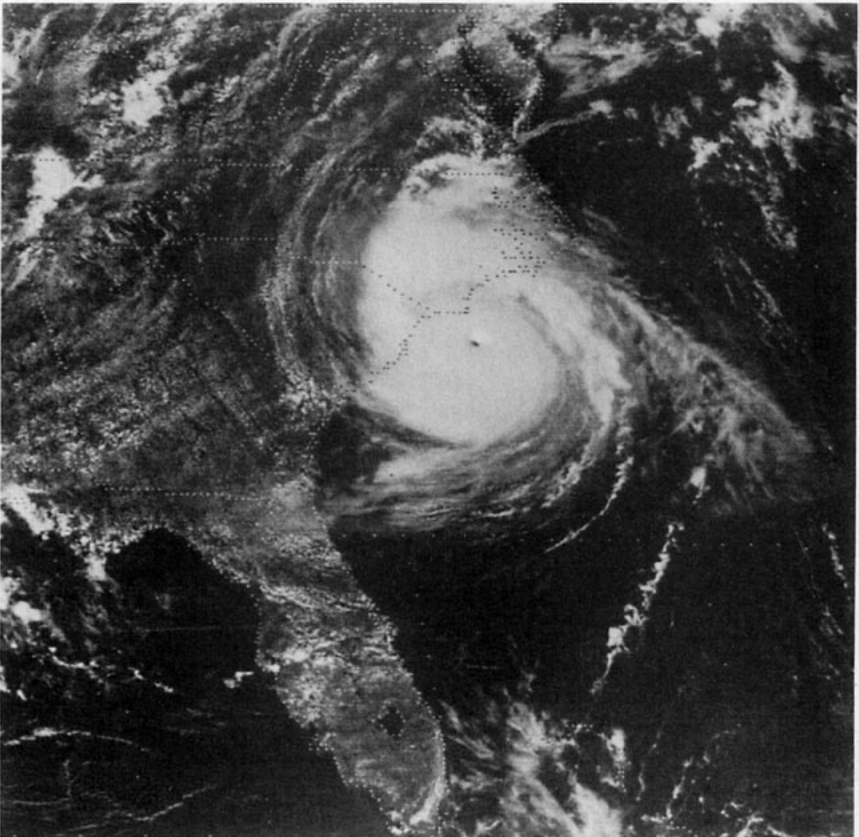
FIG. 5. GOES-West visible satellite picture of Hurricane Diana at 1900 GMT 11 September 1984. The well-defined eye is located near Cape Fear, North Carolina.
