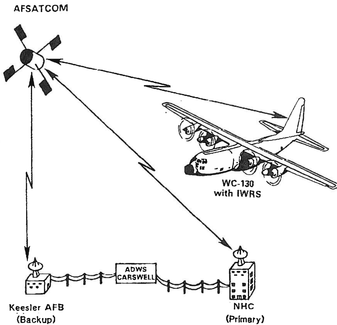
Figure 5-10. Schematic of aircraft to satellite data link for AFRES WC-130 aircraft
