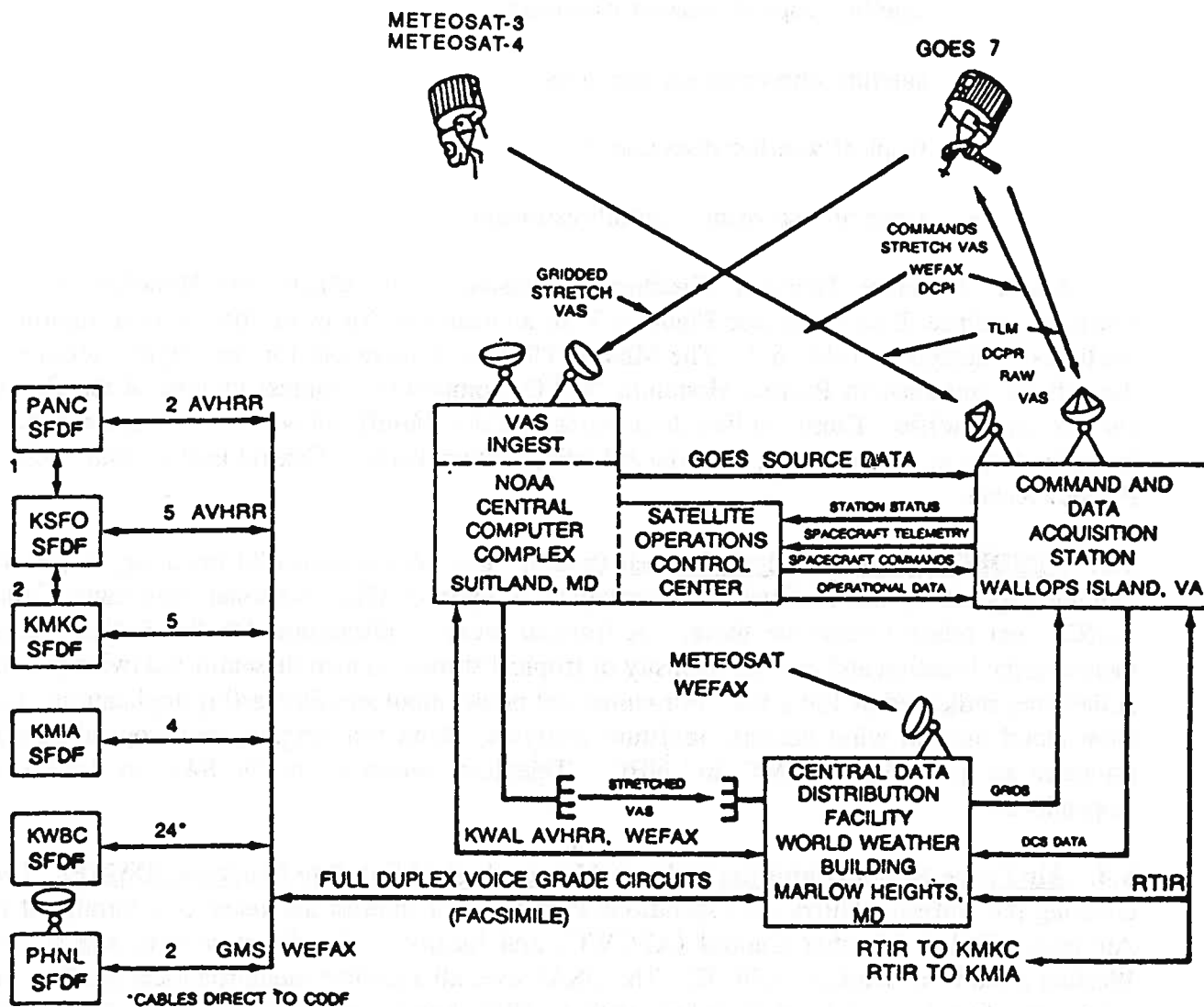
Figure 6-2. GOES central data distribution system
