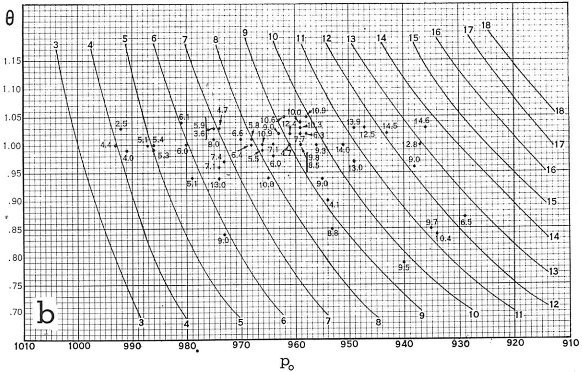
Figure 4. - (a) Storm surge prediction chart. (b) Prediction chart including dependent data.
