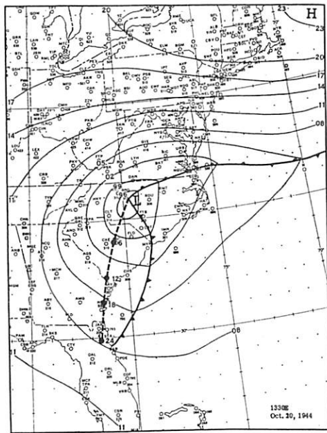
Figure 5b. - Synoptic maps of the storm center at 1330 EST, October 18-21, 1944.
