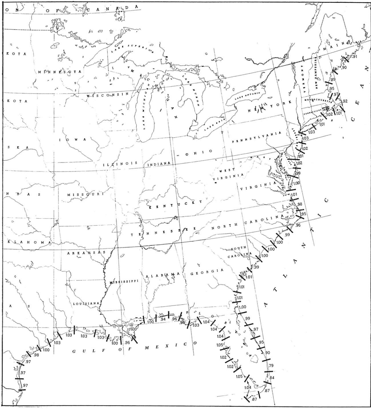
Figure 3. - Map showing relative storm surge potential \theta of various coastal sections. (See text)
