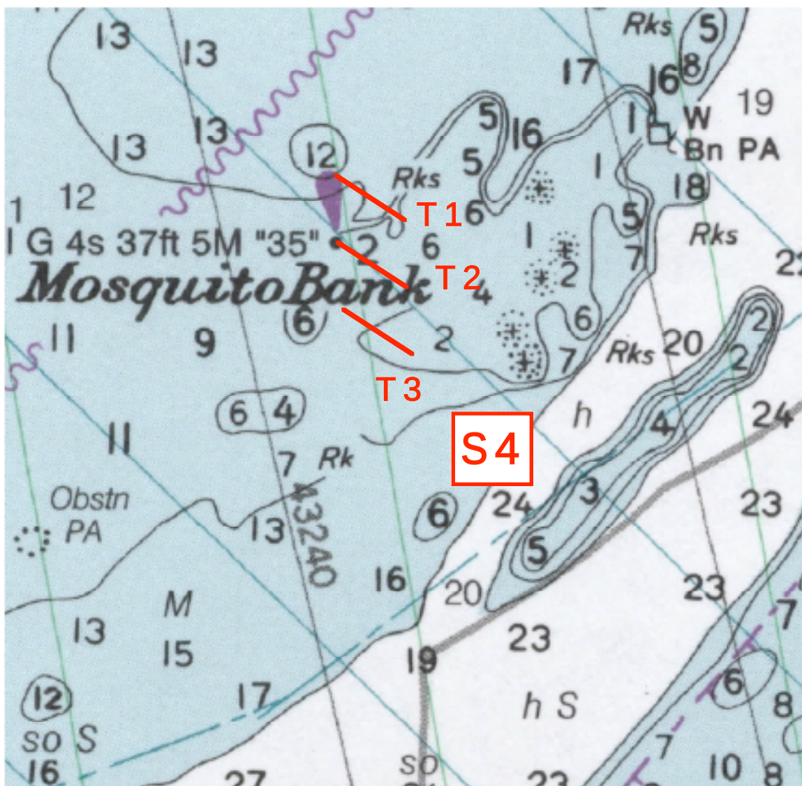
Figure 9. Location of transects. Site 4. Mosquito Bank (National Ocean Survey Chart 11462).
