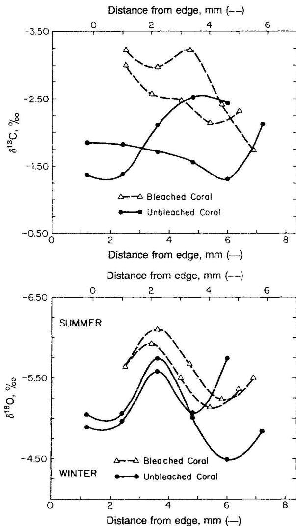
FIG. 3. Stable isotopic profile of ^{13}\text{C}/^{12}\text{C} and ^{18}\text{O}/^{16}\text{O} ratios from M. annularis across approximately 1 yr of skeletal growth. Scales for bleached coral (---) and unbleached coral (—) data are offset in order to align \delta^{18}\text{O} peaks and facilitate comparison. (Upper) \delta^{13}\text{C} value versus distance from the coral surface. Depleted \delta^{13}\text{C} values are recorded in bleached corals ( \Delta ) relative to unbleached corals ( \bullet ) following the summer temperature peak. This reduction in the \delta^{13}\text{C} value corresponds to the reduction in zooxanthellae density and productivity during bleaching (Table 1 and Fig. 1) and indicates that the preferential removal of ^{12}\text{C} by photosynthesis has decreased (29, 30). (Lower) \delta^{18}\text{O} values versus distance from coral surface. Depleted (more negative) isotope values indicate calcification in warmer waters (summer); positive isotope values indicate calcification in cooler waters (winter). A reduction or cessation of skeletal calcification is evident in bleached corals ( \Delta ) shortly after the peak summer temperature. Note that resolution of the sampling technique cannot distinguish between reduction and cessation of calcification at the skeletal surface. In contrast, unbleached corals ( \bullet ) continued to grow, as evidenced by the deposition of aragonite with enriched (more positive) \delta^{18}\text{O} values, indicative of calcification in cooler water. Cleaned M. annularis skeletons were cut along the corallite axes into slabs 2–3 mm thick, and x-radiographed with a Philips Radifluor 360 instrument for 20 s at 60 kV to illuminate the coral bands. Sequential samples were collected at 1-mm intervals with a dental drill along 10-mm transects oriented in the direction of upward growth. Each isotopic value represents the mean of samples from three transects per colony. The data from two colonies is plotted. Aragonite samples were roasted in vacuo at 425°C for 1 hr and then treated with purified orthophosphoric acid at 60°C. The isotopic composition of the \text{CO}_2 gas generated by this reaction was determined on a VG SIRA-24 mass spectrometer (sensitivity to 50 \mu\text{g} of calcite \text{CO}_2 generated) and is presented in the \delta (‰) notation relative to the PDB (Pee Dee belemnite) carbonate standard (std) where \delta = [(R_{\text{sample}}/R_{\text{std}}) - 1] \times 10^3 and R is the ^{13}\text{C}/^{12}\text{C} or ^{18}\text{O}/^{16}\text{O} ratio, respectively.
