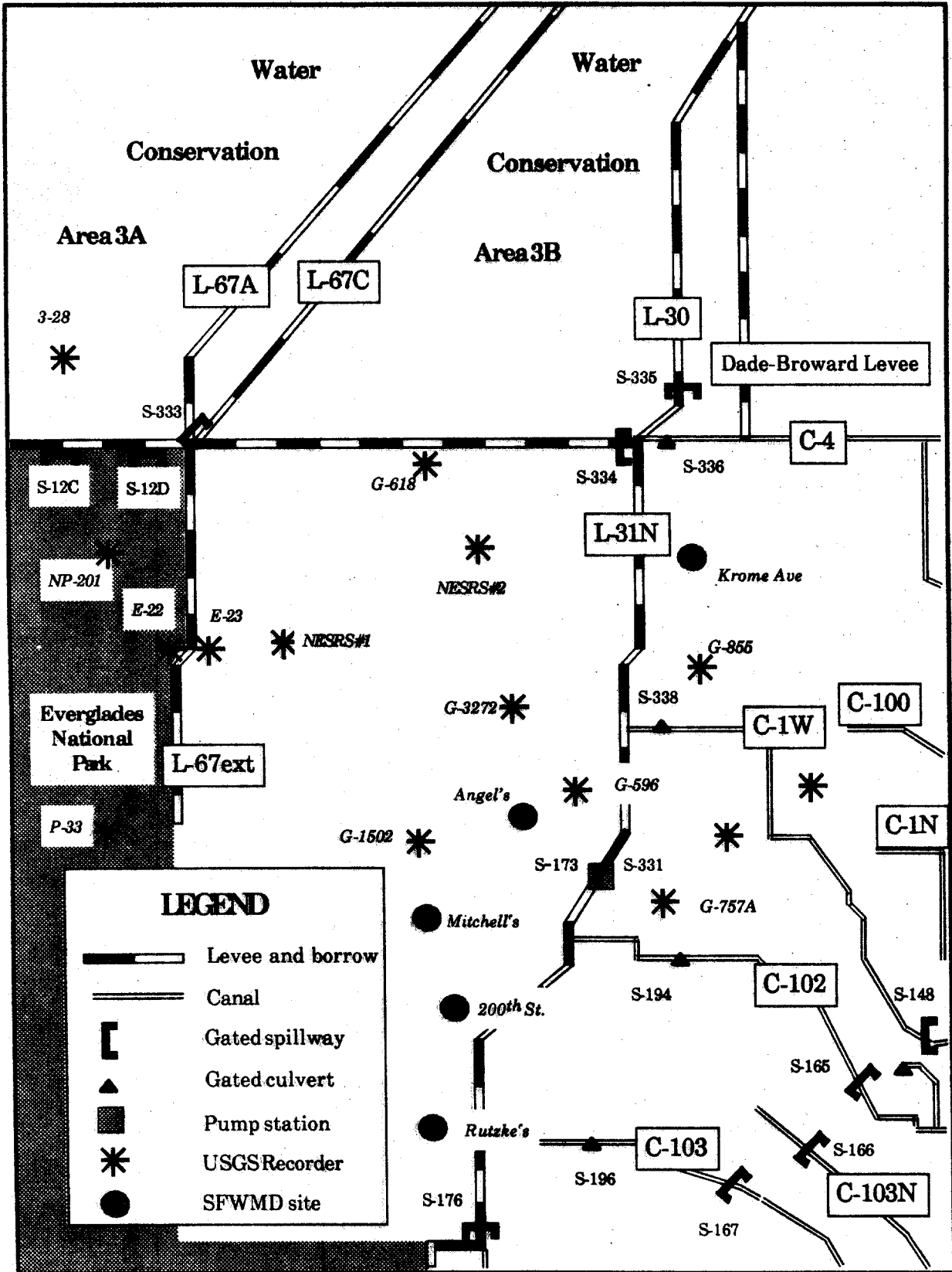
Figure 3. Daily Water Level Monitoring Network.
