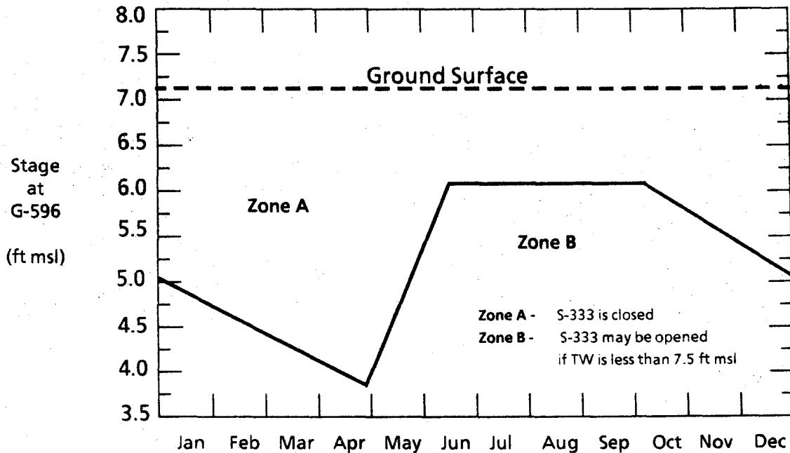
Figure 2. G-596 Schedule as a Restraint to S-333 Discharges
