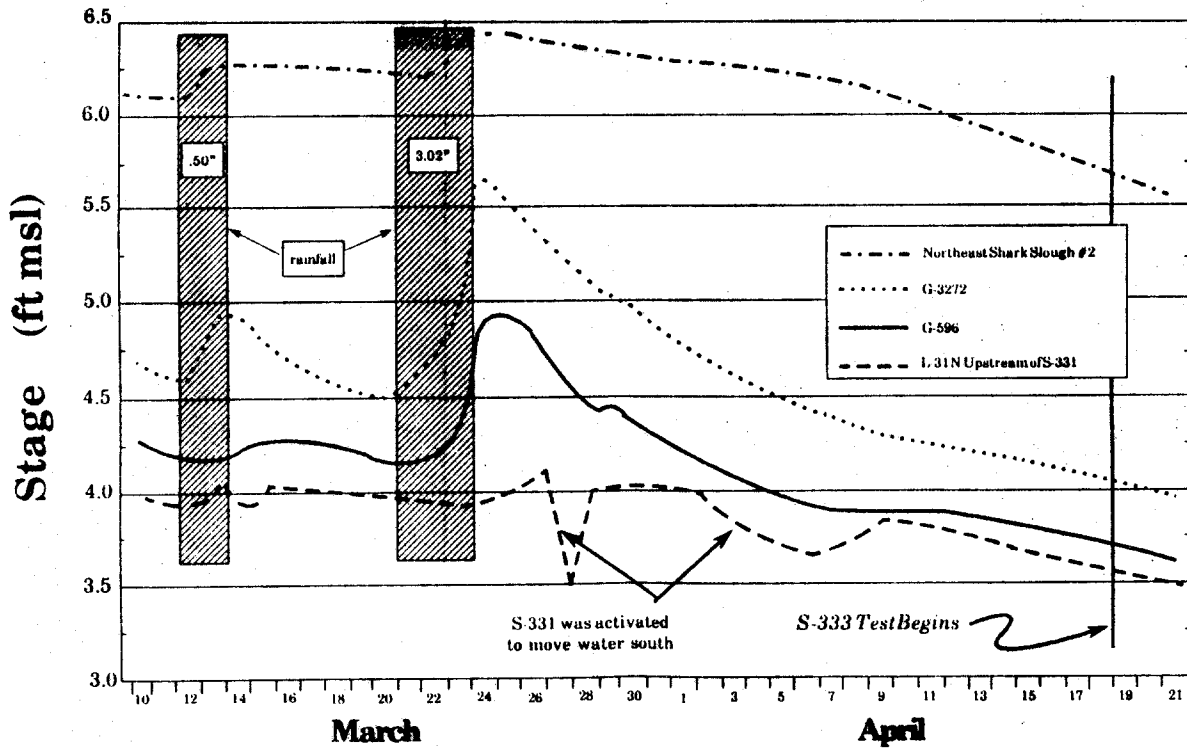
Figure 4. Pre-S-333 Test Conditions. (Note the rapid response to rainfall at all locations and the sharp drop in the L-31N canal upstream of S-331 when the pumps are turned on.)
