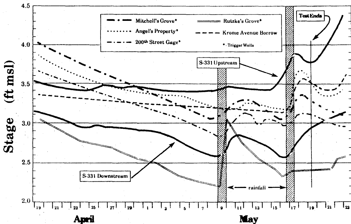
Figure 9. Hydrologic Response of New Monitoring Points Established for the Test. (Rutzke's Grove is 7 miles south of S-331 and the water table is controlled by the L-31N canal north of S-176. The water table in the Frog Pond is controlled by the L-31W and C-111 canals.)
