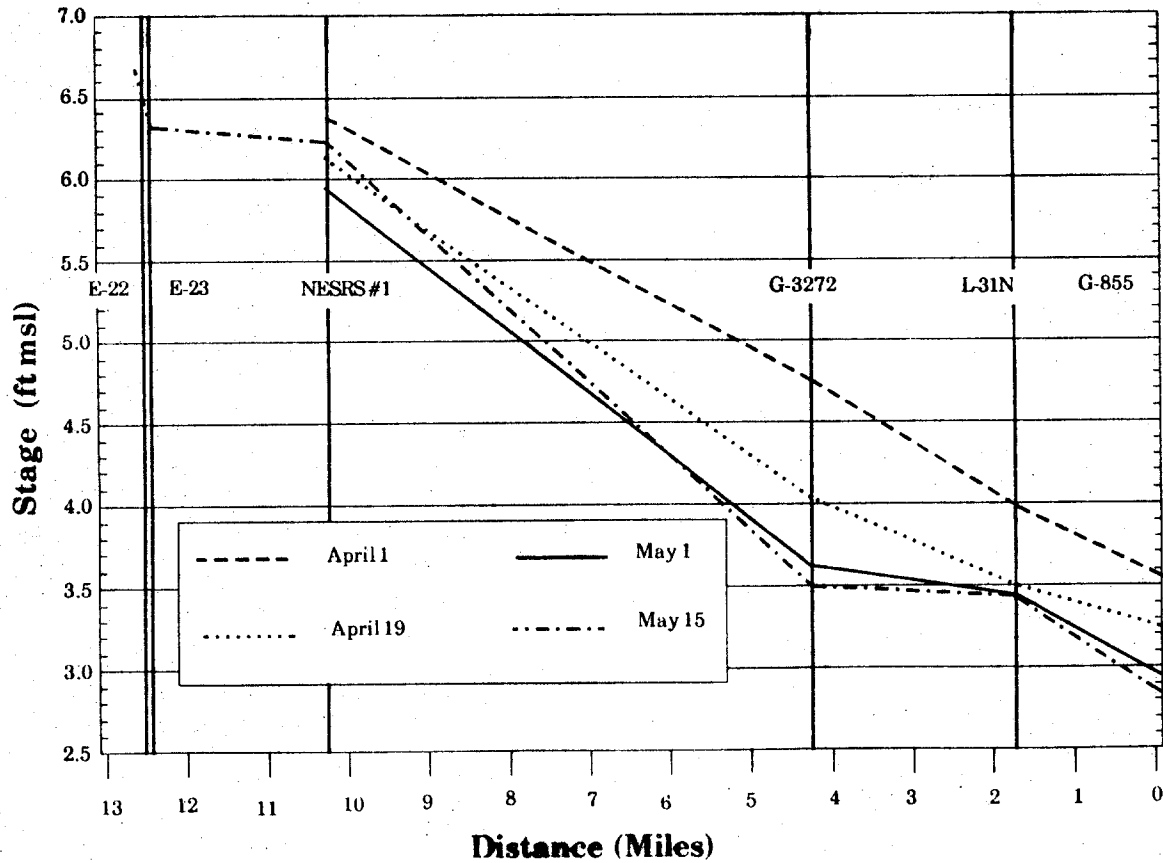
Figure A4. Transect B, through Northeast Shark River Slough from L-67ext to well G-855 (east of L-31N)
