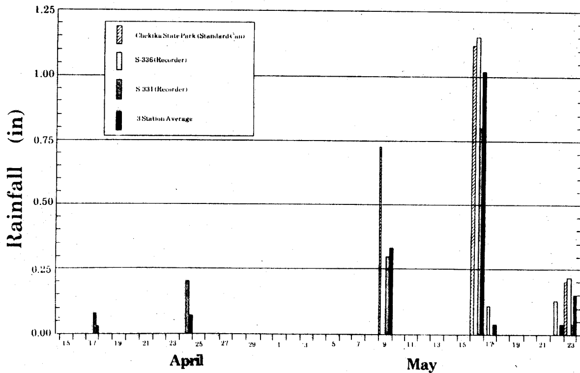
Figure 6. Rainfall During S-333 Discharge Experiment
