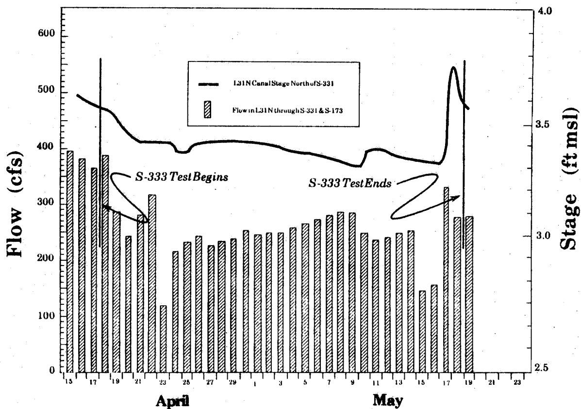
Figure 10. There was no canal inflow to L-31N during the test period. The discharge through S-331 and S-173 comes entirely from groundwater flow into the canal between S-335 and S-331.
