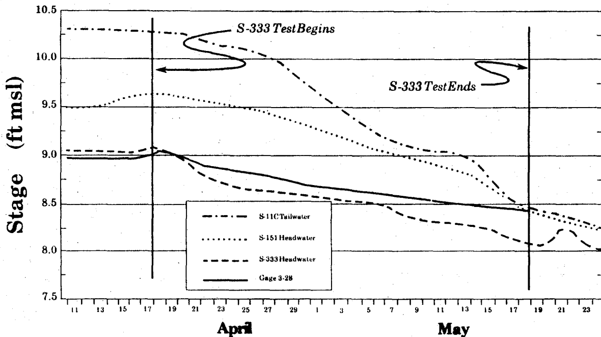
Figure 11. The response of water levels in WCA-3A is a result of the 30-day S-333 field test. S-333, S-151, and S-11 are all connected by a canal and respond quickly. Gage 3-28 is a marsh gage 2.5 miles from the canal. It responds more slowly, but was definitely influenced by the discharge through S-333.
