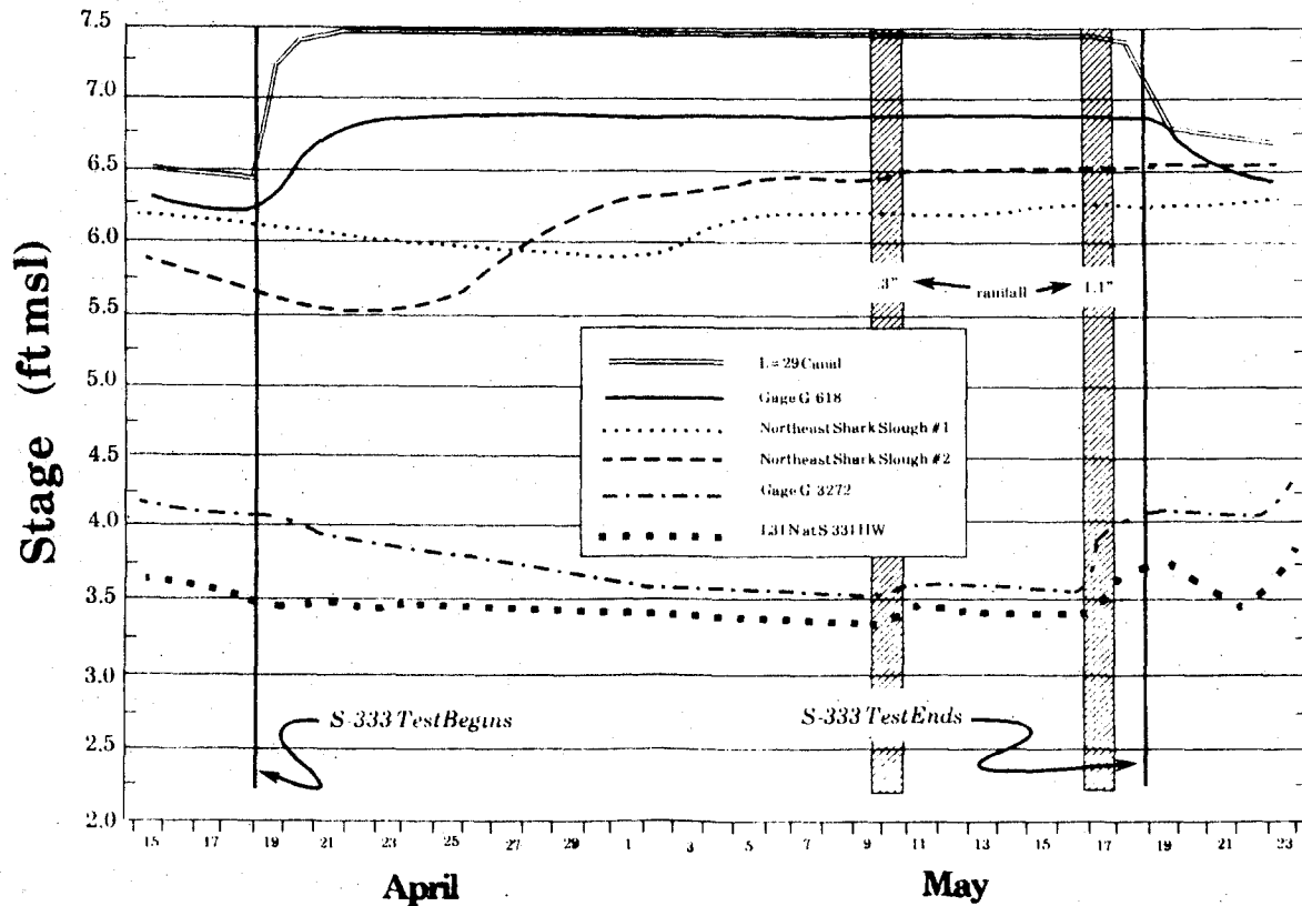
Figure 7. Water Surface Elevations at Selected Stations in the East Everglades. (The Northeast Shark River Slough surface water gages all showed marked increases, while the groundwater monitoring points showed no change due to S-333.)
