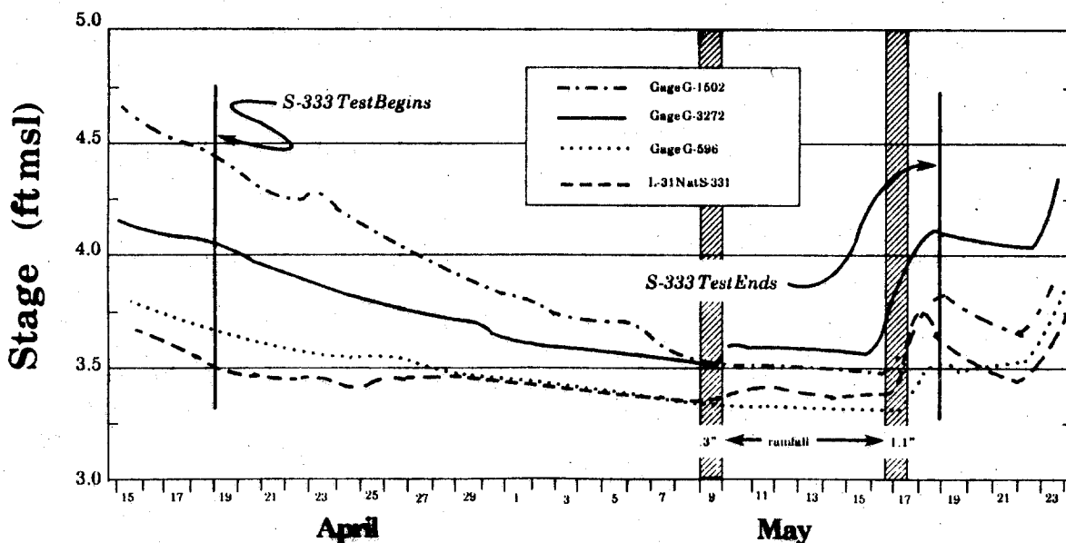
Figure 8. Groundwater Stages in the Rocky Glades west of L-31N. (All gages follow the L-31N stage closely and show no increase traceable to S-333 activity.)
