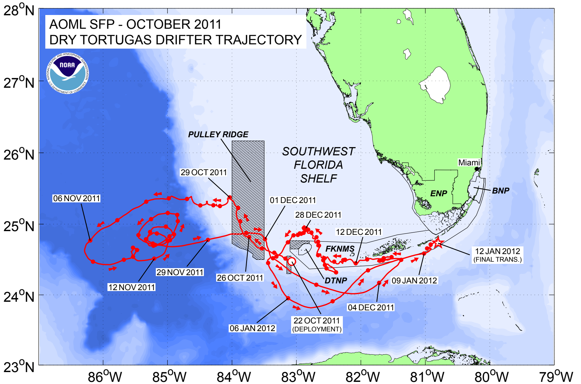
CODE Drifter #945719 deployed at Riley's Hump in the Tortugas Ecological Reserve South (TERS) on 22 October 2011.
