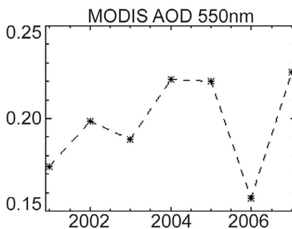
FIG. 2.24. Time series of annual mean AOD over the Amazon basin from MODIS.
