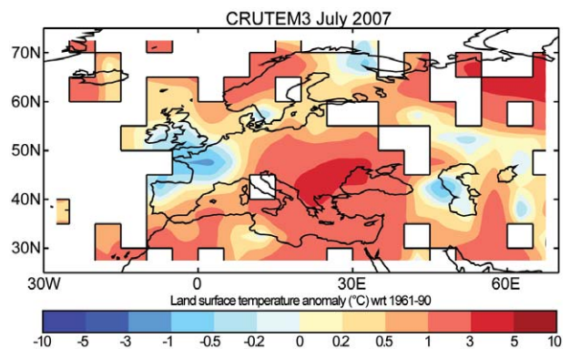
FIG. 6.47. European land surface air temperature anomalies (°C; relative to 1961–90) for Jul 2007 from the CRUTEM3 dataset (Brohan et al. 2006).
