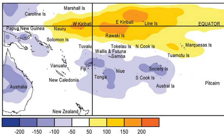
FIG. 6.54. OLR anomalies ( W m^{-2} ; 1971–2000 base period). High radiation levels (yellow or orange) are typically associated with clearer skies and lower rainfall, while cloudy conditions lower the OLR (blue) and typically mean higher rainfall.
