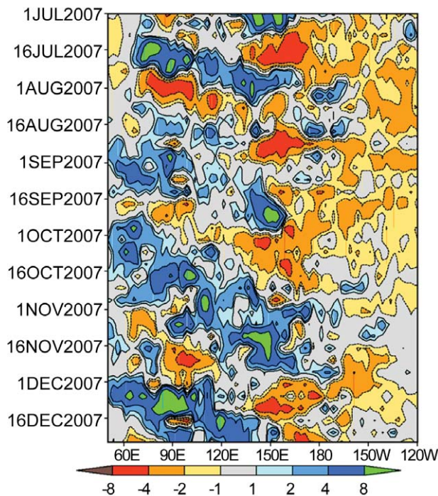
FIG. 2.12. Time-longitude section of precipitation anomaly averaged over the tropical Pacific (5°S–5°N) as observed by the GPCP pentad precipitation dataset (Xie et al. 2003). Precipitation anomaly is calculated using 1979–95 as the base period.
