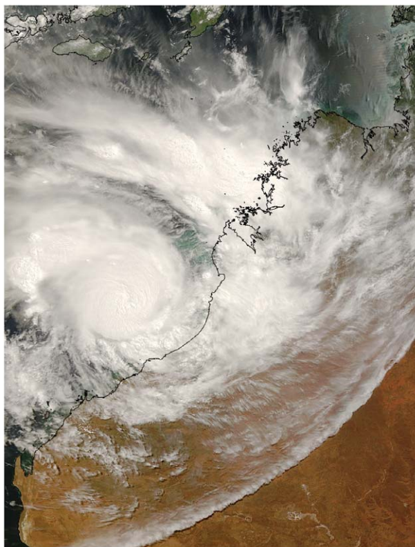
FIG. 4.26 Tropical Cyclone George approaching the coast of western Australia at 0155 UTC, 8 Mar 2007. [Courtesy of MODIS Rapid Response Project at NASA's Goddard Space Flight Center.]
