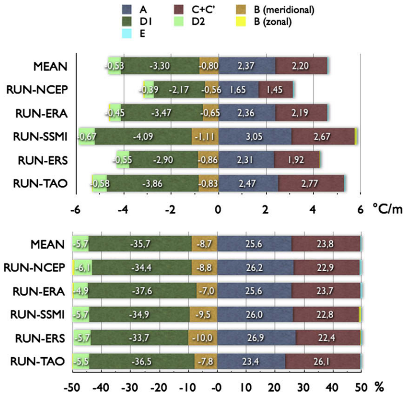
Fig. 7. Mean 1993–2000 SST tendencies for the five simulations, and for their mean, averaged in the 160–90°W, 2°S–2°N box. The atmospheric forcing ( A ) is in dark blue; the entrainment through the base of the mixed layer ( D2 ) is in light green and the turbulent mixing ( D1 ) in dark green. The mean zonal advection (part of term B ) is in yellow, the mean meridional advection (part of B ) in orange, and the advection by the eddies ( C + C' ) in red. Diffusion ( E ) is in light blue. Top: in °C per month. Bottom, in percentage of the total heat exchanges. Associated numerical values are indicated only when the percentage is higher than 1%. (For interpretation of the references to colour in this figure legend, the reader is referred to the web version of this article.)
