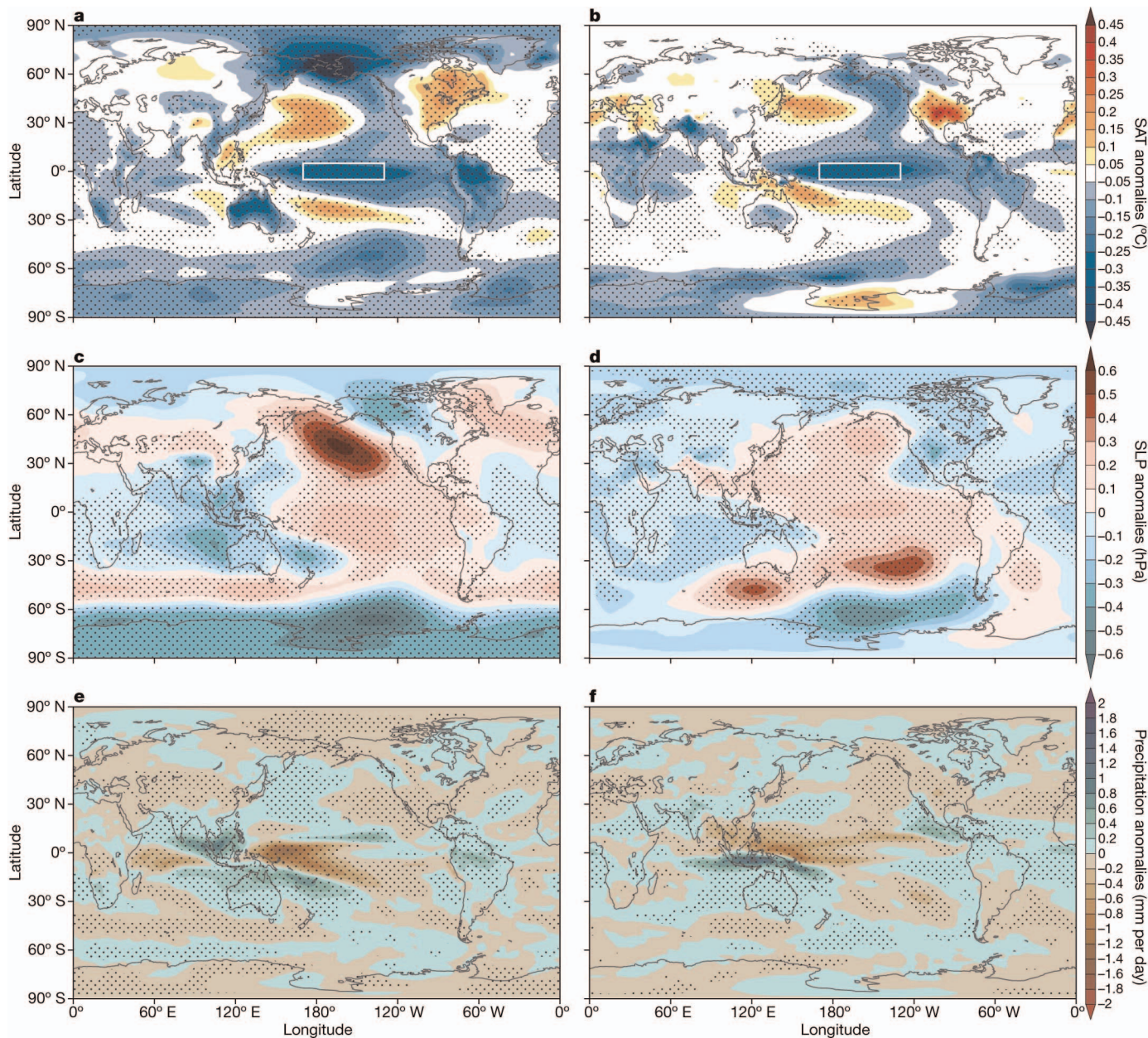
Extended Data Figure 5 | Decadal anomalies associated with SST cooling over the equatorial Pacific. Low-pass-filtered intermember anomalies in HIIST regressed against SST anomalies over the area denoted by 5° S–5° N and 170° E–130° W (white boxes in a and b). a, b, SAT; c, d, SLP; e, f, Precipitation for DJF (a, c, e) and JJA (b, d, f). The sign is flipped to show a La Niña state.
