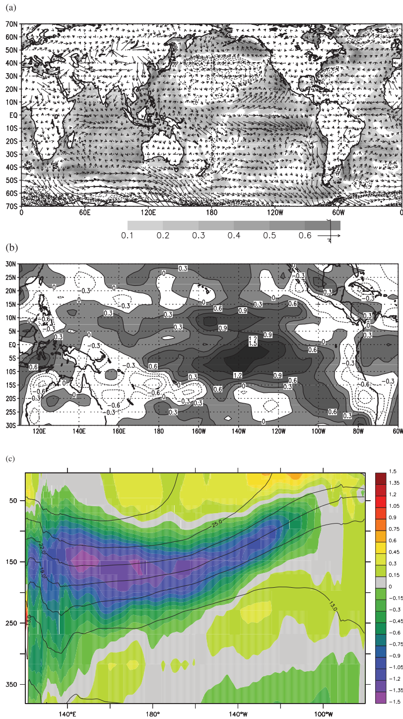
Figure 17. (a) Long-term changes in mean SST (°C) and winds at 1000 hPa (m/s), obtained by subtracting the mean SST of the period 1958–1978 from that over the period 1979–2004. (b) Long-term changes in annual mean zonal winds at 1000 hPa (m/s), obtained similar as to Figure 17a. (c) Differences of ocean temperature in two periods of 1958–1978 and 1979–2004 along with the depth-longitude section of climatological ocean temperature (black contours).
