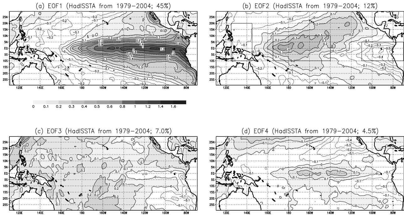
Figure 2. Top four EOF modes of tropical Pacific SSTA (1979–2004) multiplied by respective standard deviations of the principal components; units in ^{\circ}\text{C} .
