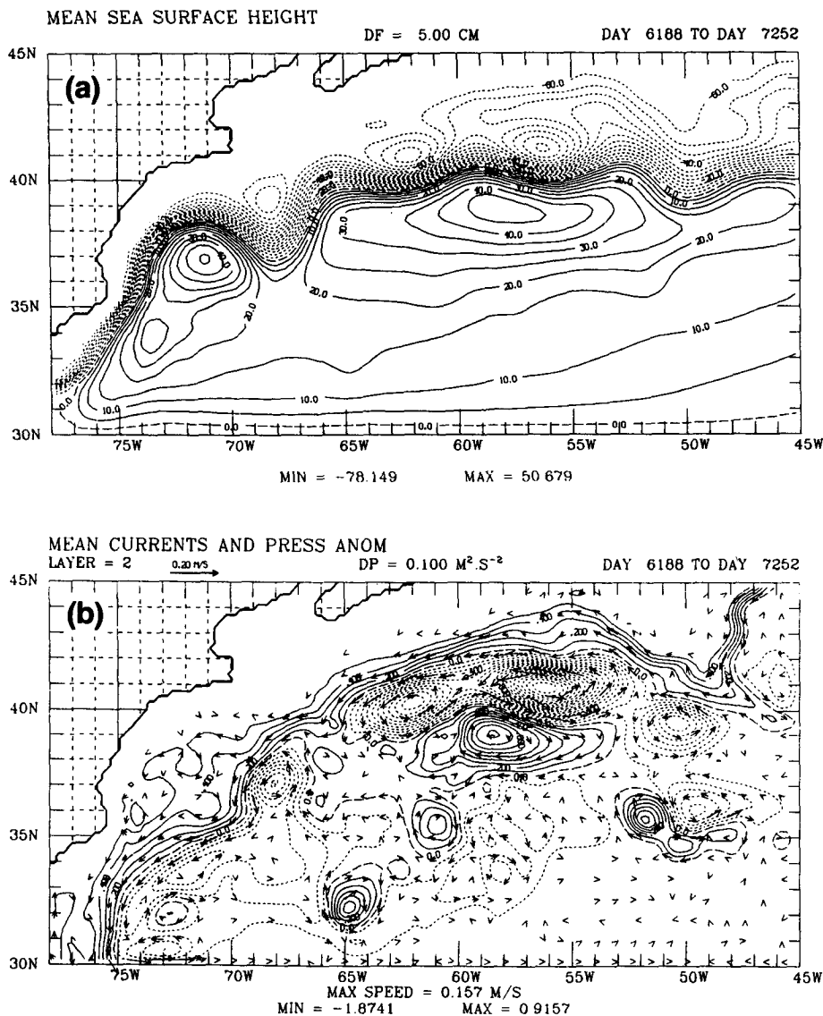
FIG. 10. As in Fig. 8 but for Experiment 5a.
