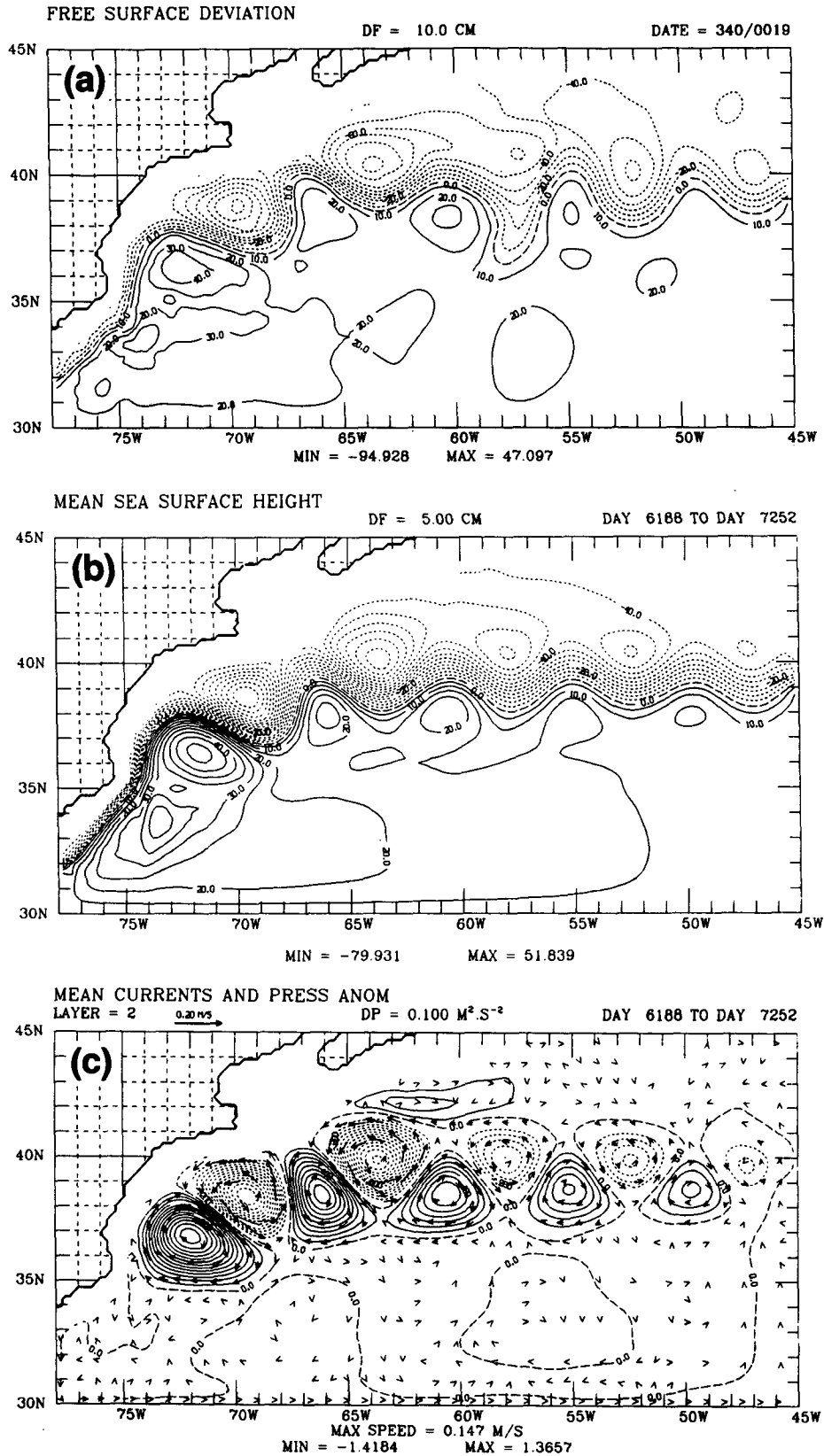
FIG. 5. Results from Experiment 2 for: (a) SSH at year 19, Day 340. Contour interval is 10 cm. (b) Mean SSH (5 cm contour interval). (c) Deep mean currents and mean PA2 (0.1 m 2 s -2 contour interval).
