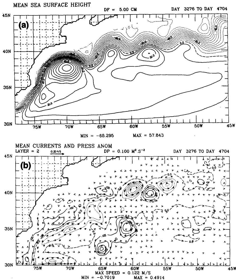
FIG. 8. Experiment 4 (a) mean SSH. Contour interval is 5 cm. (b) Deep mean currents and mean PA2. Contour interval is 0.1 m s -2 .
