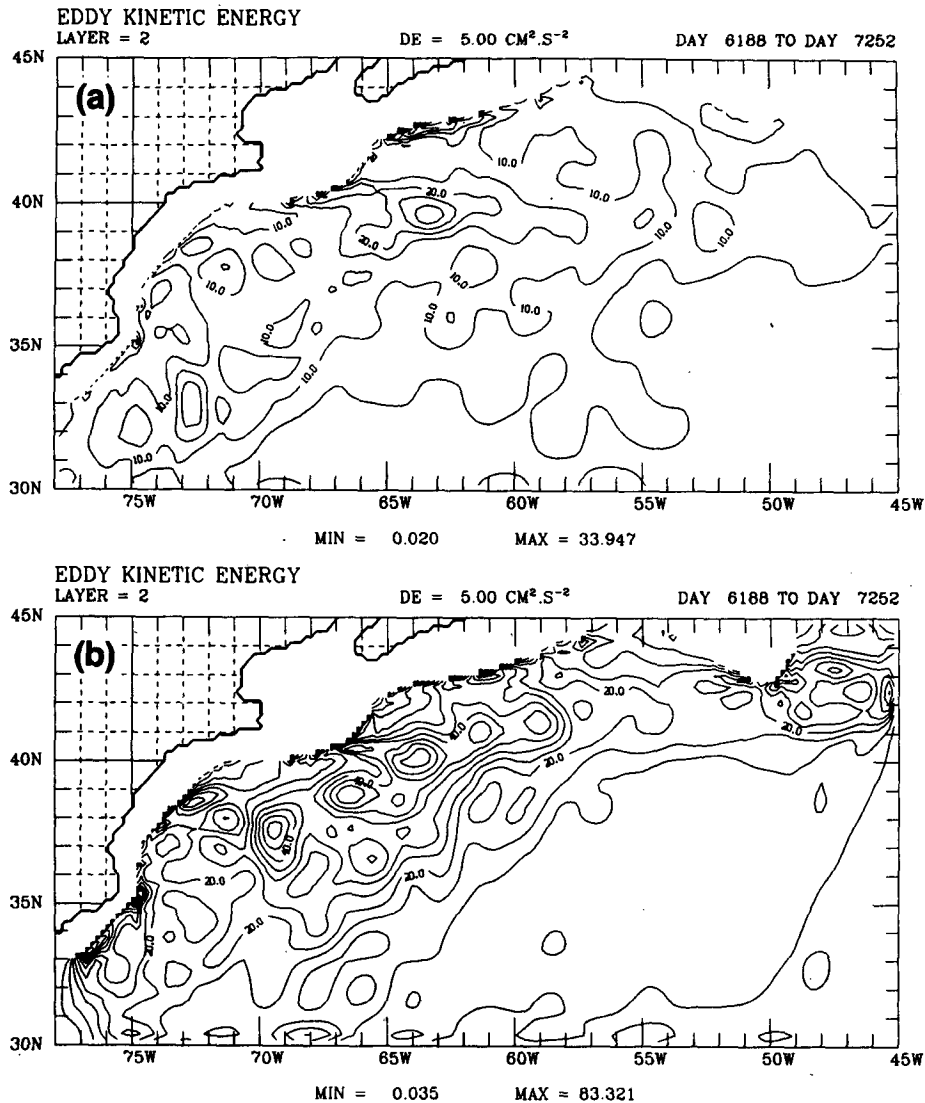
FIG. 7. (a) EKE2 for Experiment 2. (b) EKE2 for Experiment 3. Contour interval is 5 \text{ cm}^2 \text{ s}^{-2} .
