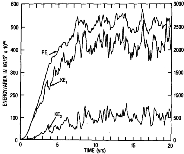
FIG. 9. Time series of basin-averaged potential energy per unit area due to thermocline (model interface) fluctuations and upper and lower layer kinetic energy per unit area in units of \text{kg s}^{-2} . Scale on the left refers to kinetic energy while scale on the right refers to potential energy.
