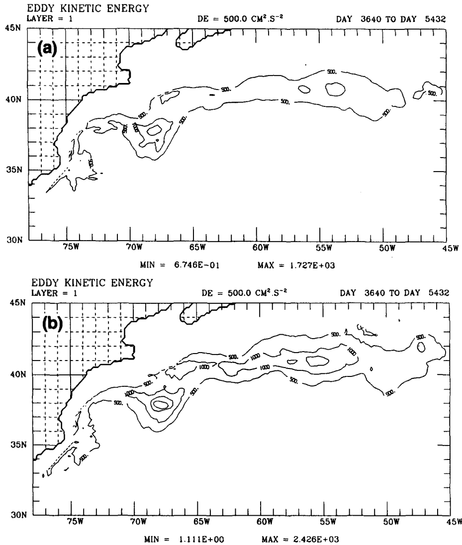
FIG. 14. EKE1 from (a) Experiment 5a and (b) Experiment 5b. Contour intervals are 500 cm 2 s -2 .
