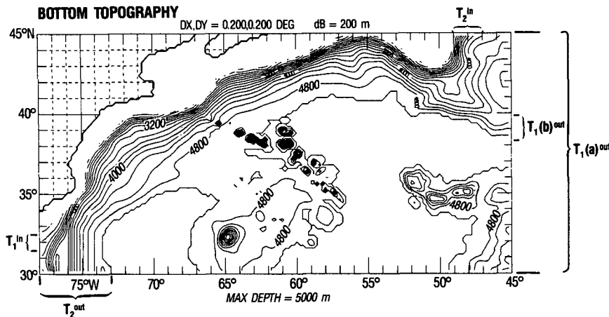
FIG. 2. Model domain for the limited-area Gulf Stream model. Bottom depths are shown with a 200 meter contour interval. Inflow ( T_i^{in} ) and outflow ( T_i^{out} ) location for upper ( i = 1 ) and lower ( i = 2 ) layer transports are also noted.
