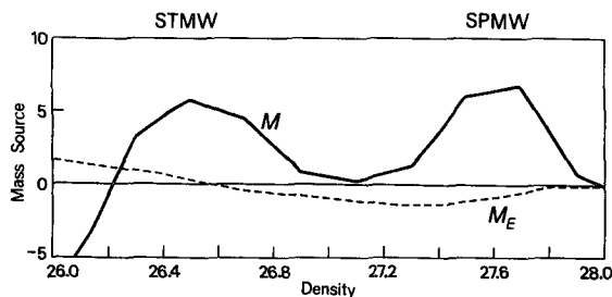
FIG. 4. Mass source ( \times 10^6 \text{ m}^3 \text{ s}^{-1} ) from density flux ( M ) and Ekman pumping ( M_E ) in the upper part of the sea surface density range. The left-hand lobe is centered near the density of subtropical mode water (STMW) while the right-hand lobe spans subpolar mode water (SPMW) and Labrador Sea Water densities.
