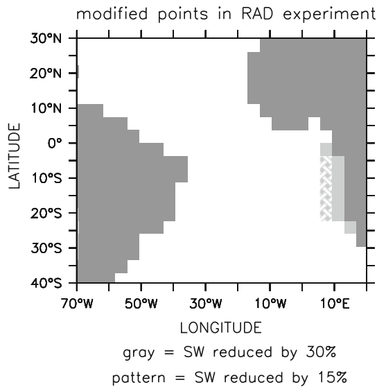
Fig. 2 Model grid points where modifications in the RAD run are applied as denoted on the figure, for details see text
