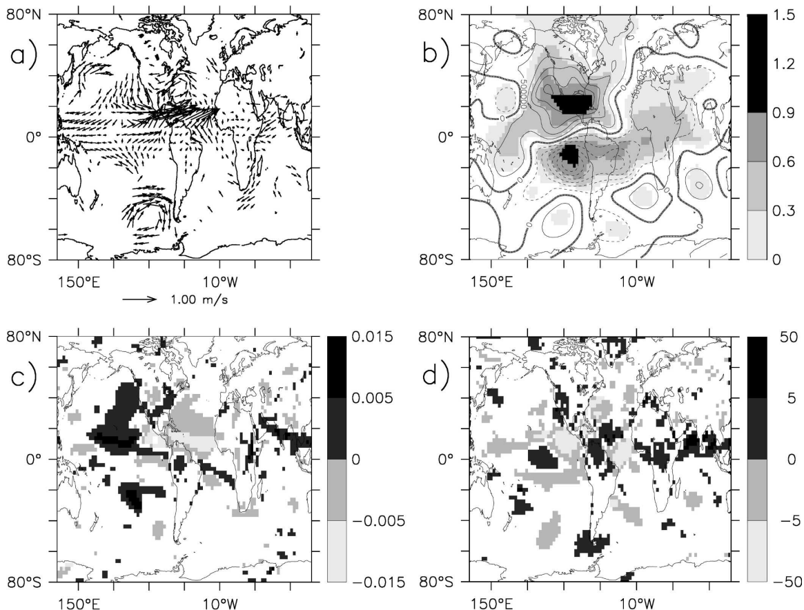
FIG. 8. Atmospheric response to warming of the North Atlantic ( NA^+ - NA^- ) in JJA. Same as in Fig. 3, but for (a) 1000-hPa winds. Only regions where at least one component of the wind is significant at the 95% level are shown. (b) 200-hPa streamfunction. Shaded regions are significant at the 95% level and show signal to noise ratio. (c) Omega at 500 hPa. Units are \text{Pa s}^{-1} . Negative values denote ascent. (d) Total heat flux into the ocean. Units are \text{W m}^{-2} .
