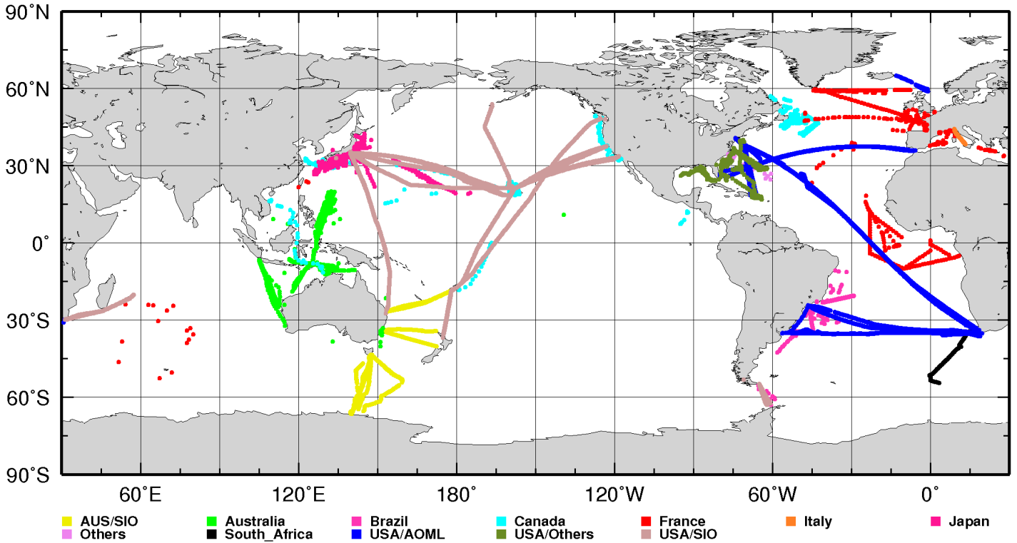
XBT Transmissions Y2018 (Total 15983)
