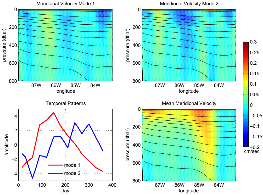
Figure 3: Principal components (lower-left panel), 1st EOF (upper-left) and 2nd EOF (upper-right) for the meridional velocity, and mean meridional velocity at the southern open boundary. The inserts show the bathymetry at the open southern boundary.
