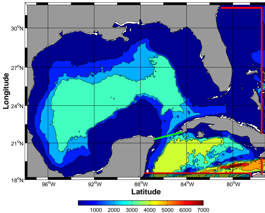
Figure 1: Model domain. Color-filled contours indicate bathymetry in meters. Computational information from larger domain is provided along the red line along the open boundary. Uncertainty of the inflow is modeled in the cross-hatched region at the southern boundary.
