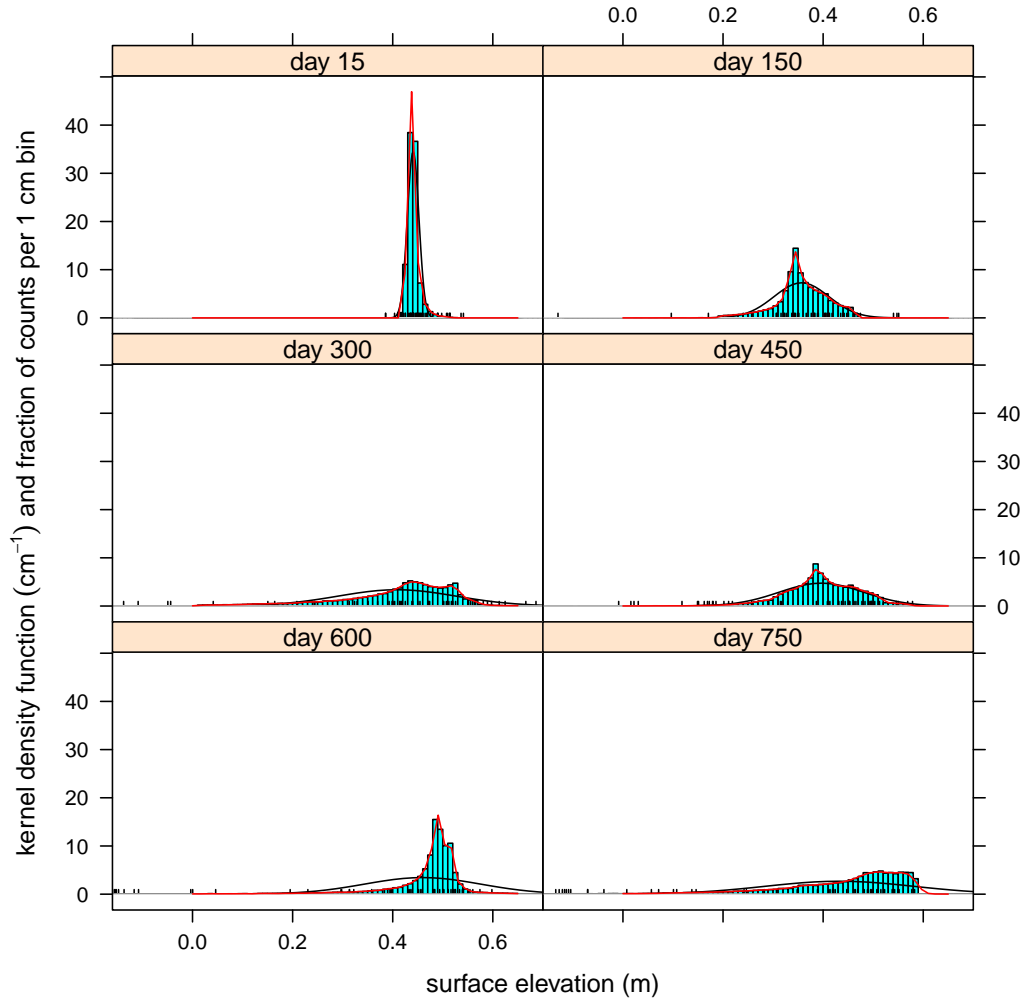
Figure 10: Kernel density estimates for surface elevation ( m ) at the point ( 86^{\circ}\text{E} , 24.1^{\circ}\text{N} ) for days 15, 150, 300, 450, 600, and 750. They were derived from histograms generated using polynomial chaos expansion for the mixed layer depths corresponding to 50,000 random boundary conditions. Ticks along the bottom indicate values for the 49 HYCOM simulations. Red curves are kernel density estimates, and black curves are Gaussian densities with means and standard deviations from the polynomial expansions.
