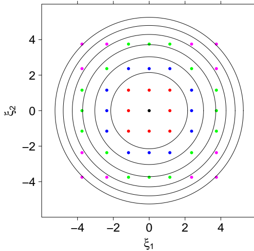
Figure 4: Circles enclose regions of 90%, 99%, ..., 99.9999% probability. Dots mark locations of the Gauss-Hermite quadrature points, with red dots corresponding to relatively likely, blue less likely, green unlikely, and magenta highly unlikely boundary conditions.
