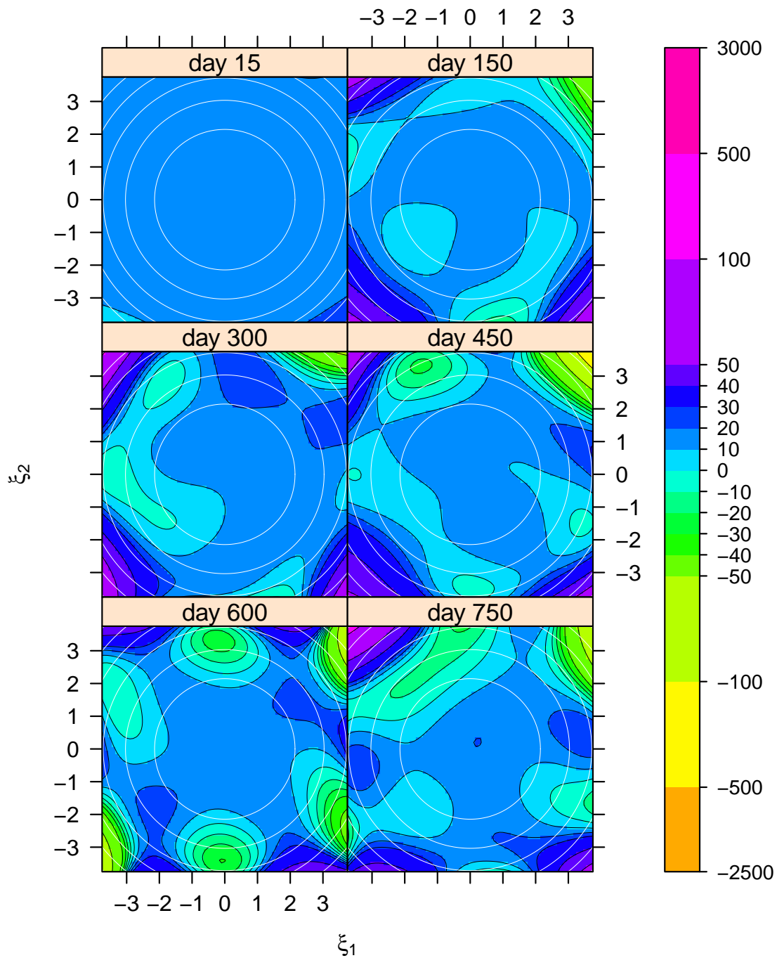
Figure 9: Surface elevation (cm) at (86°E,24.1°N) as a function of random variables \xi_1 and \xi_2 . Note the compressed color scale used to distinguish more likely from less likely responses: Contours are at 10 cm intervals from -50 to 50 cm, and more extreme values are represented with a compressed scale. The circles, which are the same as those of figure 4, indicate that the extreme values are highly unlikely.
