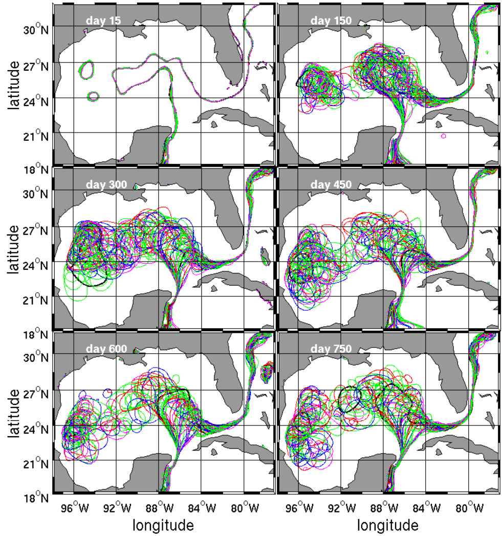
Figure 5: Locations of the Loop Current and its eddies from the 49 HYCOM quadrature runs as indicated by 17 cm sea-surface-height contours. The panels, from upper left to lower right, show the contours at 15, 150, 300, 450, 600, and 750 days after the boundary uncertainties were initiated. The colors of the contours correspond to the colors of the dots in figure 4 with the thick black contour indicating the central member of the ensemble.
