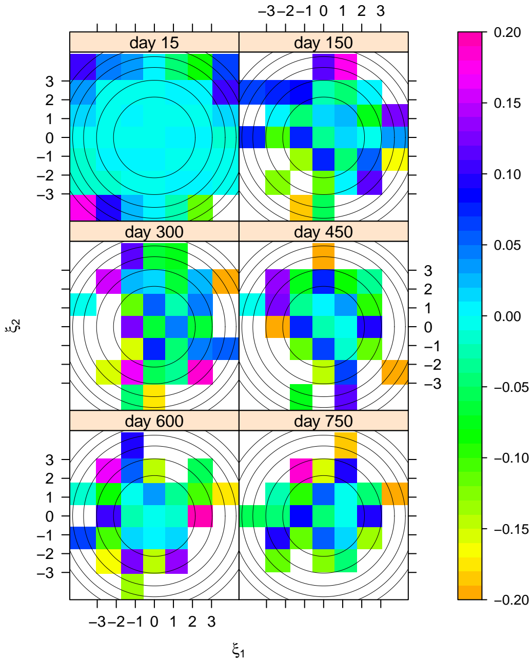
Figure 12: Errors (m) of the polynomial chaos expansion for sea-surface-height at (86°E,24.1°N). The color of each rectangle indicates the difference between the HYCOM simulation and its approximation by the polynomial chaos expansion at each quadrature point, with white indicating errors larger than 20 cm. The circles are contours of the probability density function as in figure 4.
