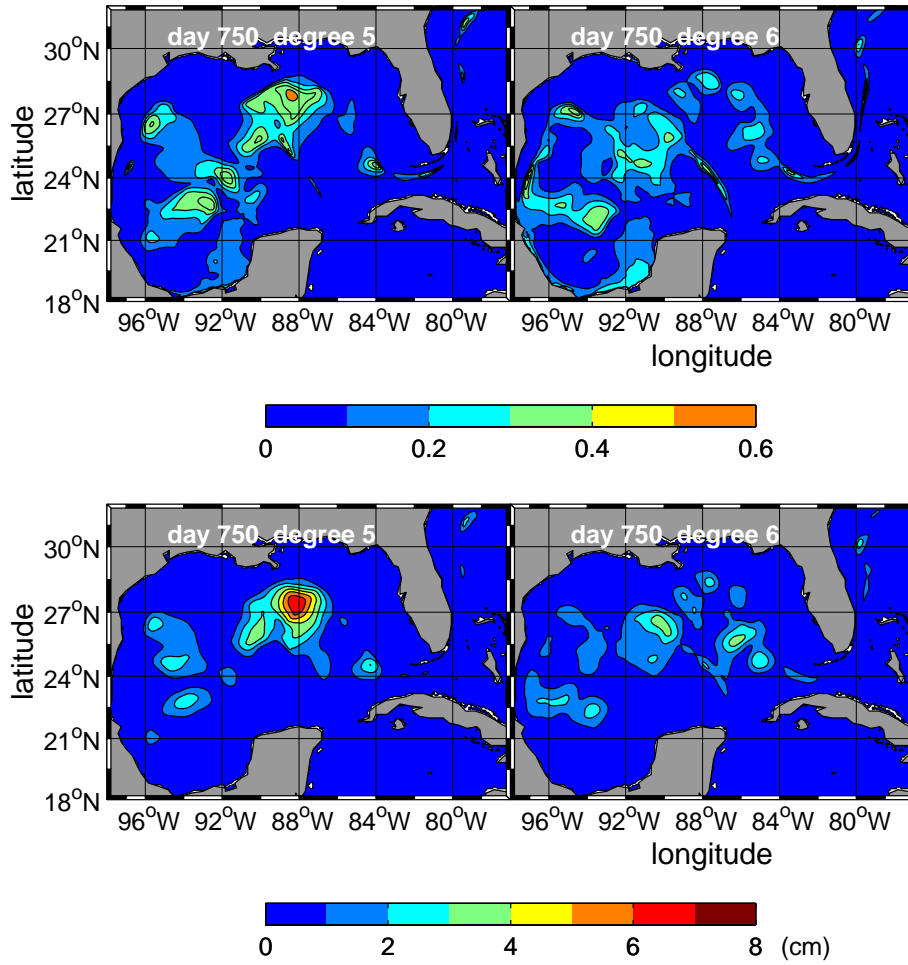
Figure 11: Upper panels show fraction of variance of surface elevation at day 750 due to the retained polynomial terms of highest degree: (left) contribution of the 6 5th-degree terms relative to the total contributed by the 21 terms of degree less than 6; (right) contribution of the 7 6th-degree terms relative to the total contributed by the 28 terms of degree less than 7. Lower panels show incremental contribution to standard deviation (cm) of surface elevation at day 750.
