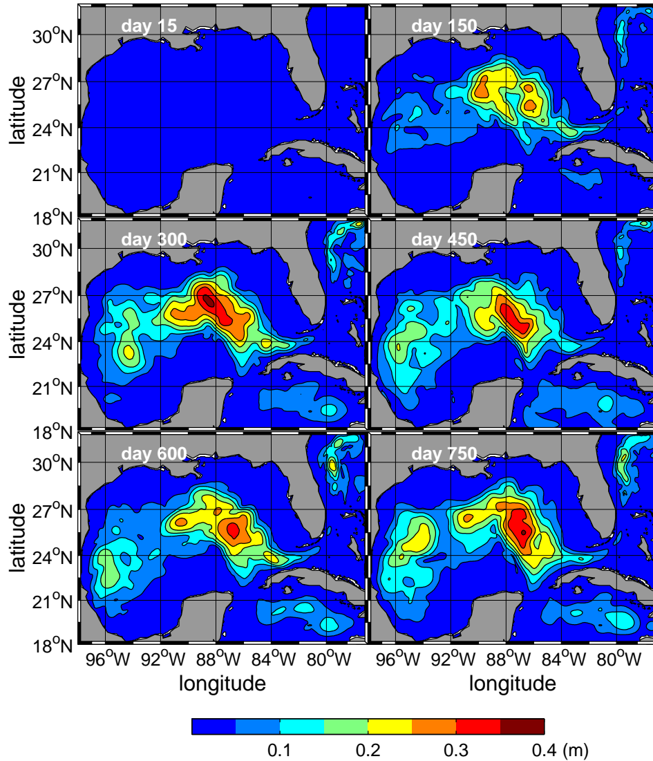
Figure 7: Standard deviation (m) of the sea-surface-height field from the polynomial chaos expansion at 15, 150, 300, 450, 600, and 750 days.
