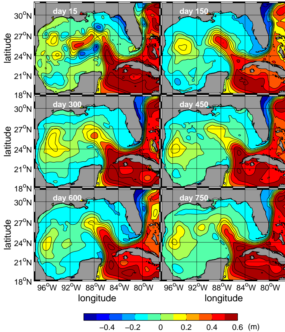
Figure 6: Mean (m) of the sea-surface-height field from the polynomial chaos expansion at 15, 150, 300, 450, 600, and 750 days after the boundary uncertainties were initiated.
