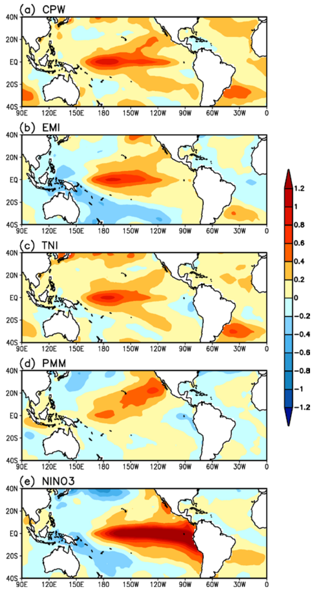
Figure 2. Composites of SST anomalies in JJASON for the eight strongest (+) phase CPW, EMI, TNI, PMM and NINO3 years. The unit is °C.
